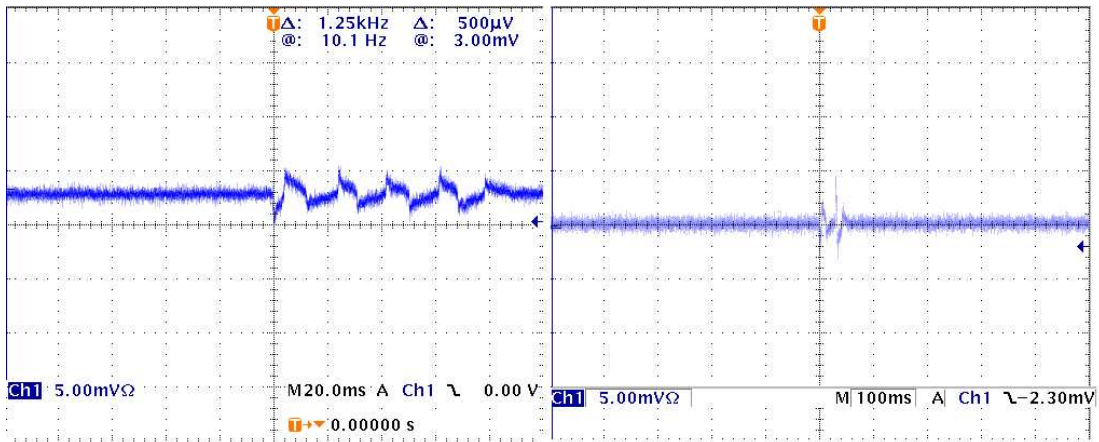
Figure 5: Current Spikes when turning off bulk power supply of MCOR 12; left: ripple peak-to-peak \approx 0.5A ; right: a spike with peaks at \approx -0.3, +0.5 A
