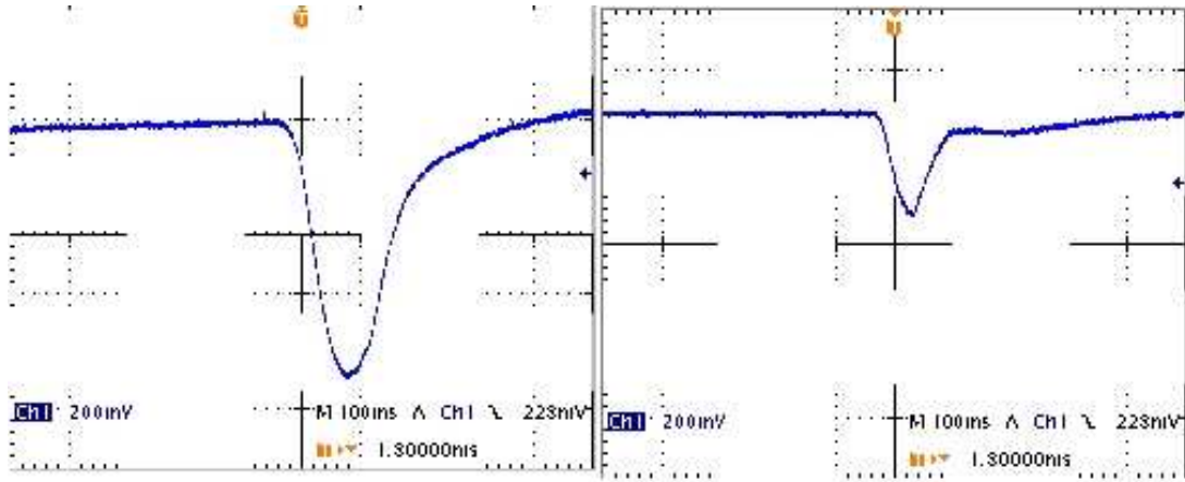
Figure 4: Current Spikes when turning off Power Supply of MCOR Calibration Stand; left: peak current -11A, right: peak current -3.75A
