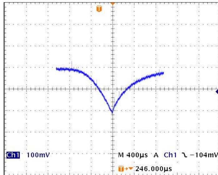
Figure 3: - 2.5A current spike when turning off Kepco power supply (100mV \sim 1.25A).
