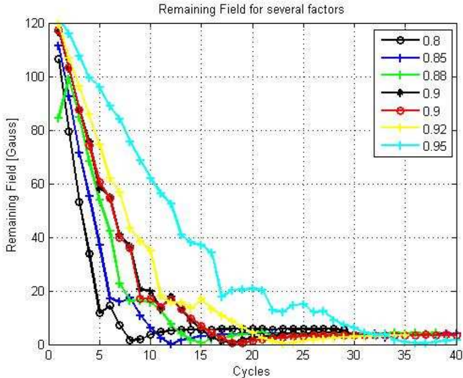
Figure 1: Remaining integrated field after cycles of degaussing.
