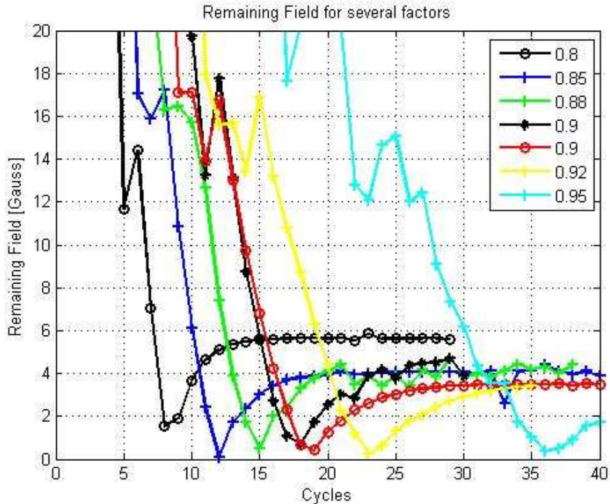
Figure 2: Remaining integrated field after cycles of degaussing.
