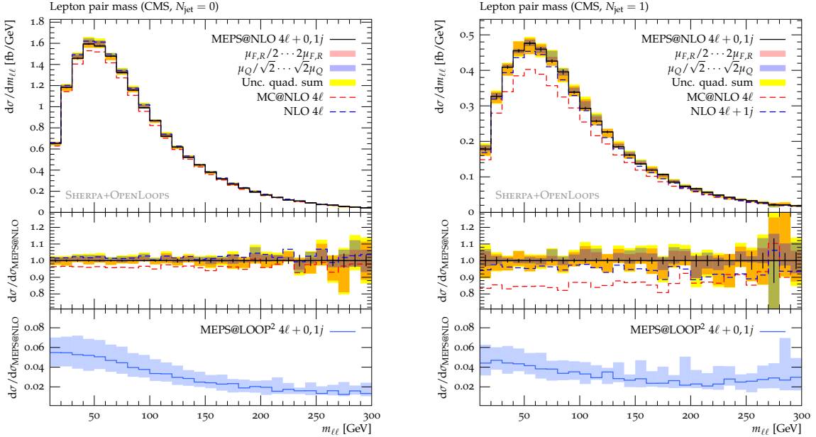
Figure 4: Invariant mass of the lepton pair in pp \rightarrow \ell^+ \ell^- + \cancel{E}_\perp + X in the exclusive zero (left) and one (right) jet selection under typical cuts used in Higgs searches. Displayed are the MEPS@NLO (black) prediction, with its associated renormalisation and factorisation scale uncertainties as well as the resummation scale uncertainty, the inclusive MC@NLO prediction and the fixed-order NLO prediction. The lower panel shows the contribution of loop induced processes to the total result.
