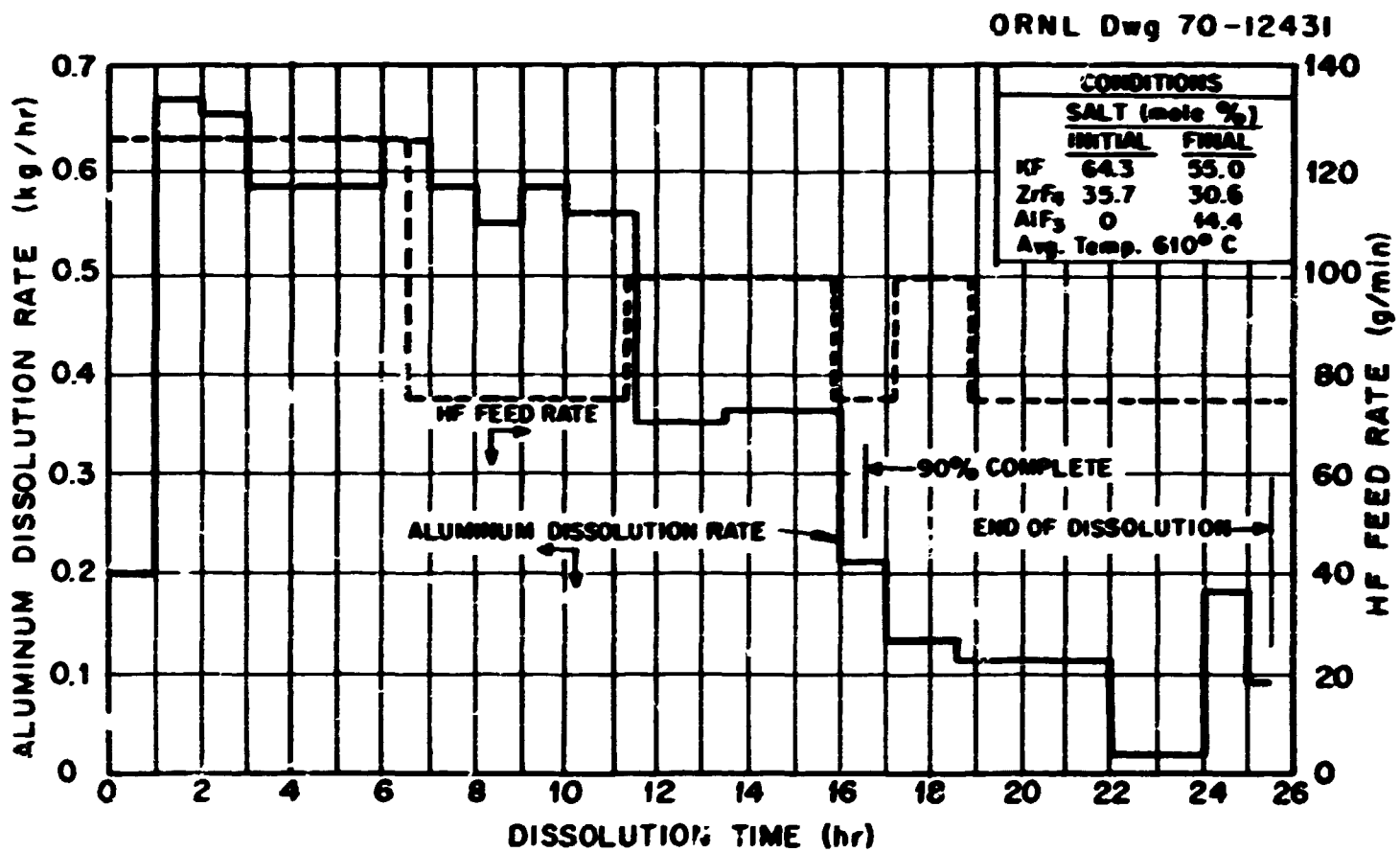
Fig. B-6. Aluminum Dissolution Rate as a Function of Fuel Element Dissolution Time for Run RA-1.
