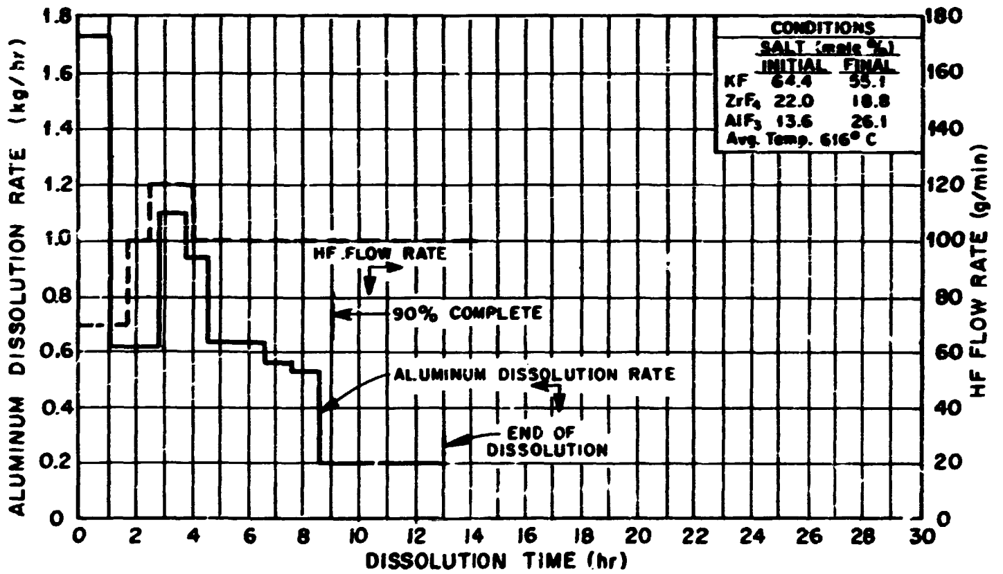
Fig. B-2. Aluminum Dissolution Rate as a Function of Fuel Element Dissolution Time for Run DA-2.
