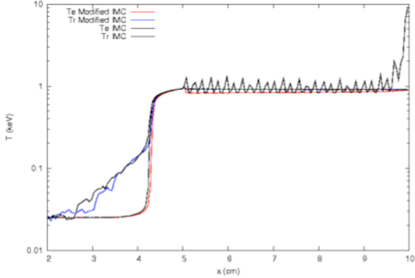
Figure 4: Fleck and Cummings IMC and modified IMC results for the radiation-hydrodynamics test problem. Matter and radiation temperature is plotted vs. space at t = 1.0 \times 10^{-7} sec. Both simulations used \Delta t = 10^{-11} sec. T_e denotes electron temperature and T_r denotes radiation temperature.
