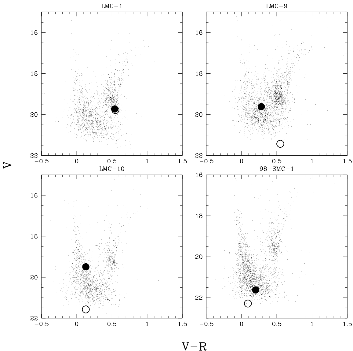
FIG. 45.—Distribution of V , V - R for \sim 3000 stars neighboring the lensed object ( filled circle ) for objects in the Magellanic Clouds. The debledned source location ( open circle ) is determined from blending parameters in the microlensing fit.
