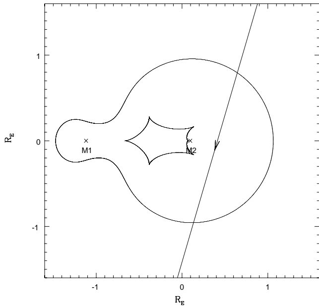
FIG. 34.—Location of the ( cuspy ) caustic and ( smooth ) critical curves for the dashed (large mass ratio) 98-BLG-14 binary lens fit ( dashed line ) presented in Fig. 32. The coordinate system, whose origin is at the center of mass, indicates distance in units of the system's Einstein Ring radius R_E . Also shown are the locations of the lensing objects, and the trajectory of the source through the caustic structure.
