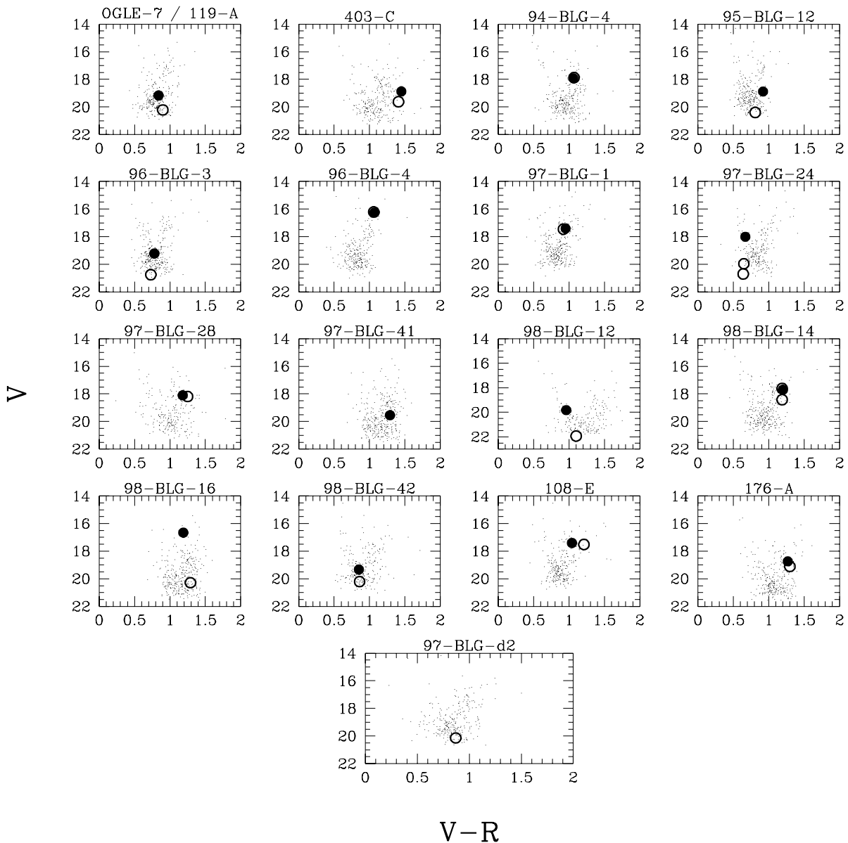
FIG. 46.—Distribution of V , V-R for \sim 3000 stars neighboring the lensed object ( filled circle ) for objects in the Galactic bulge. The debledened source location ( open circle ) is determined from blending parameters in the microlensing fit. Notable cases: 97-BLG-24, for which the brighter source is associated with the low mass ratio fit in Fig. 24; 97-BLG-41, for which we have no estimate of the source properties; 98-BLG-14, for which the brighter source is associated with the large mass ratio fit in Fig. 32; 97-BLG-d2, for which we have only an estimate of the lensed source properties.
