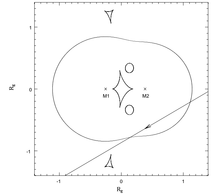
FIG. 42.—Location of the ( cuspy ) caustic and ( smooth ) critical curves for the 108-E binary lens fit presented in Fig. 41. The coordinate system, whose origin is at the center of mass, indicates distance in units of the system's Einstein Ring radius R_E . Also shown are the locations of the lensing objects, and the trajectory of the source through the caustic structure.
