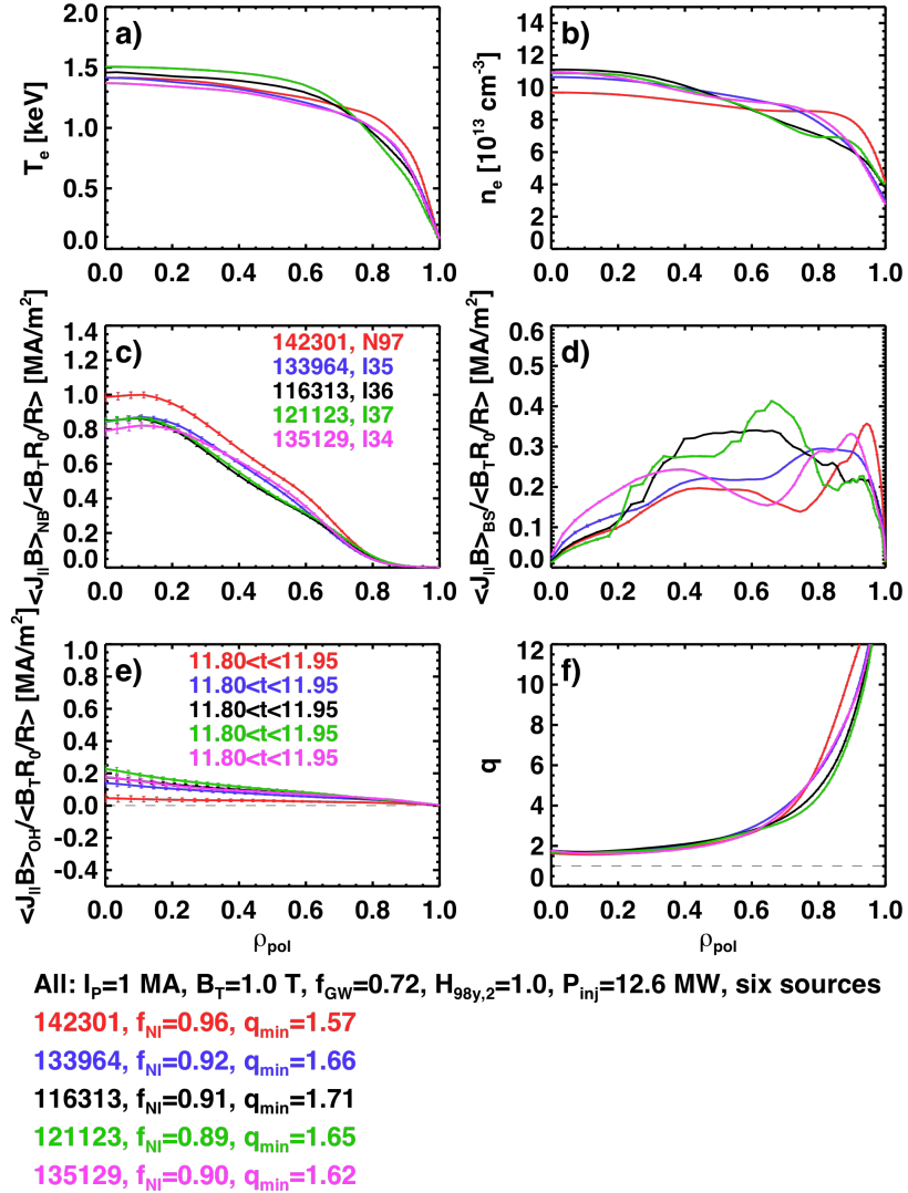
Fig. 16: Examples of how various thermal density and temperature profile shapes impact the current profile and non-inductive current level for the near non-inductive S1 scenario.
