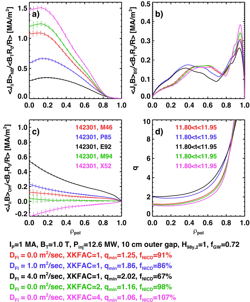
Fig. 10: Profile comparison for the S1 scenario with B_T=1.0 \text{ T} , I_p=1 \text{ MA} , H_{98y,2}=1 , with a 10 cm outer gap. The injected power is from six sources operating at 90 kV, for a total power of 12.6 MW, and the Greenwald fraction is f_{GW}=0.72 . The different curves correspond to various levels of spatially uniform fast ion diffusivity D_{FI} or multiplier XKFAC on the ion thermal diffusivity.
