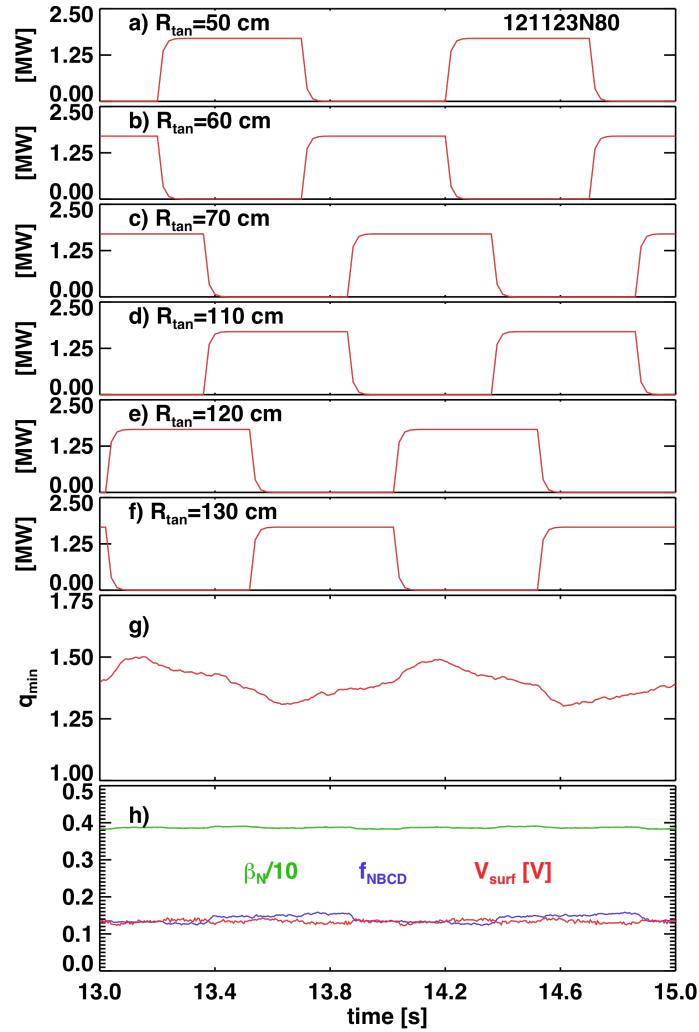
Fig. 21: Effect of neutral beam modulations on the fully evolved very long pulse scenario. Shown are the neutral beam powers in frames a)-f), the minimum safety factor ( q_{min} ) in frame g), and the normalized beta ( \beta_N ), beam current drive fraction ( f_{NBCD} ) and surface voltage ( V_{surf} ) in frame h).
