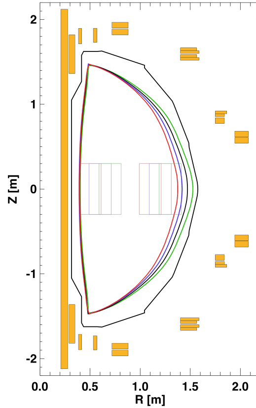
Fig. 5: High-triangularity, double-null, target shapes used in the outer gap scan. Also note the projections of the neutral beam footprints.
