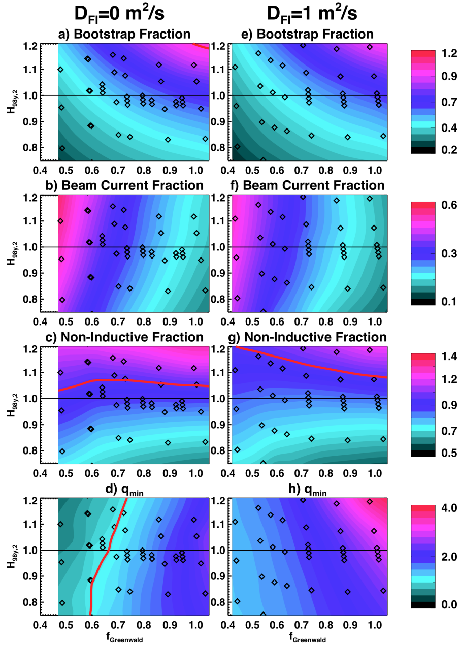
Fig. 9: Comparison of the nearly 100% non-inductive SI scenario without (left) and with (right) anomalous fast ion diffusion. The rows show the bootstrap fraction, NB current fraction, the total non-inductive fraction, and the central safety factor.
