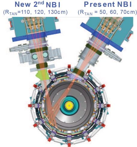
Fig. 1: Illustration of the present neutral beam injector utilized in NSTX, and the 2 nd neutral beam injector that is a primary component of the NSTX-Upgrade project.
