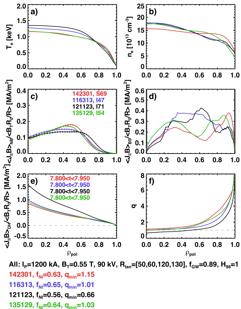
Fig 17: Effect of the various profile assumptions on the high- \beta_T scenario S3.
