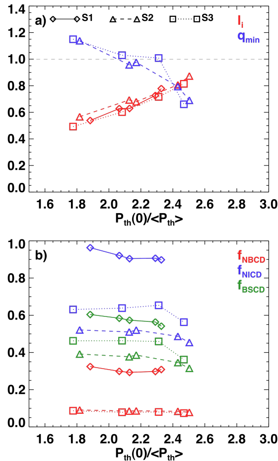
Fig. 18: Various parameters as a function of the thermal pressure peaking factor, for the S1-S3 scenarios of table #1. Frame a) shows the internal inductance and minimum safety factor, while frame b) shows the non-inductive current components.
