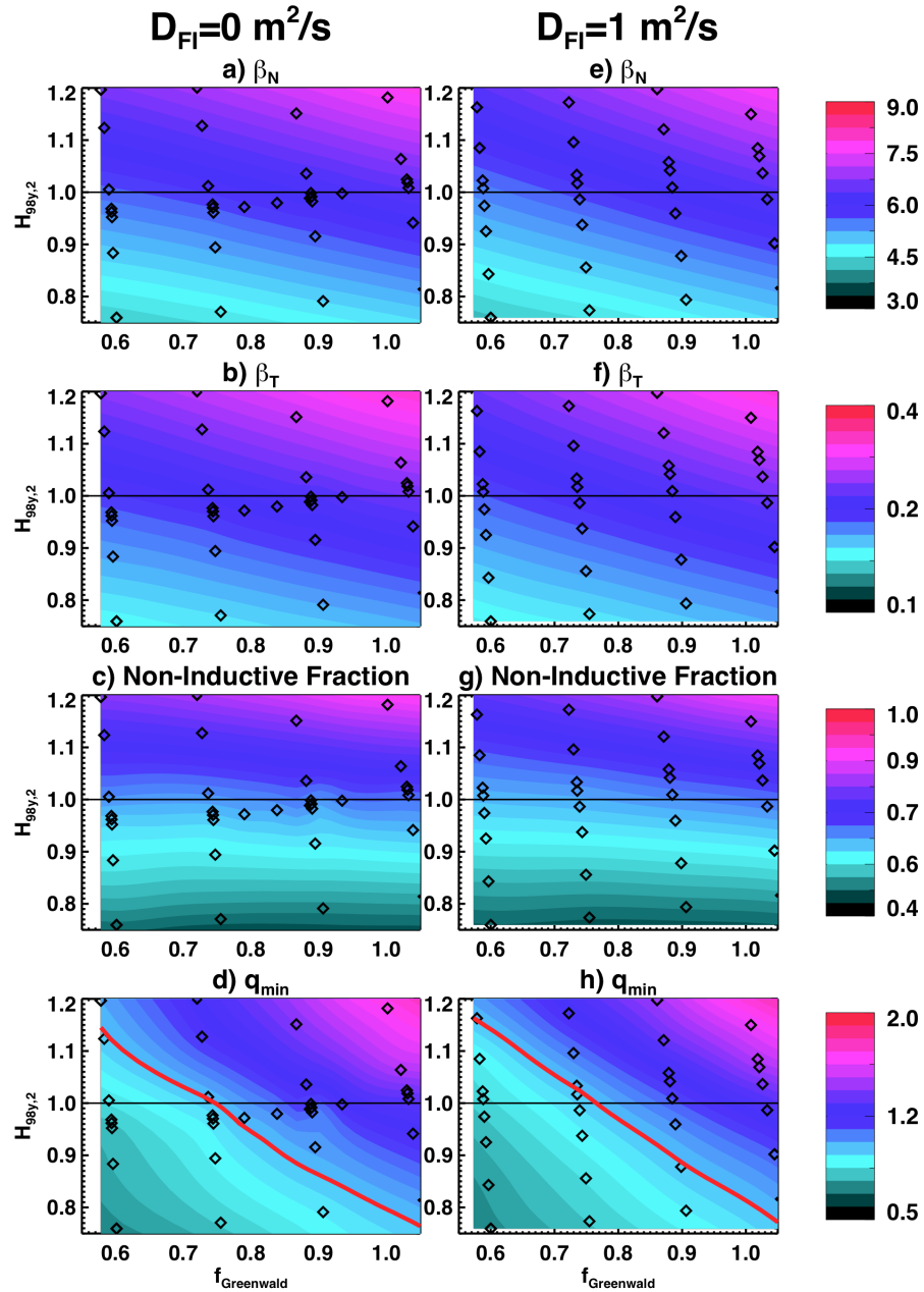
Fig. 24: Contours of \beta_N , \beta_T , the non-inductive fraction, and q_{min} vs. the confinement factor H_{98y,2} and Greenwald fraction. These configurations have I_P=1200 kA, B_T=0.55 T with R_{tan}=[50,60,120,130] , 90 kV beams and a target boundary shape with A=1.81 and \kappa=2.95 . The left column has D_{FI}=0 m 2 /s, while the right column has D_{FI}=1 m 2 /s. The q_{min}=1 contour is illustrated in the bottom row.
