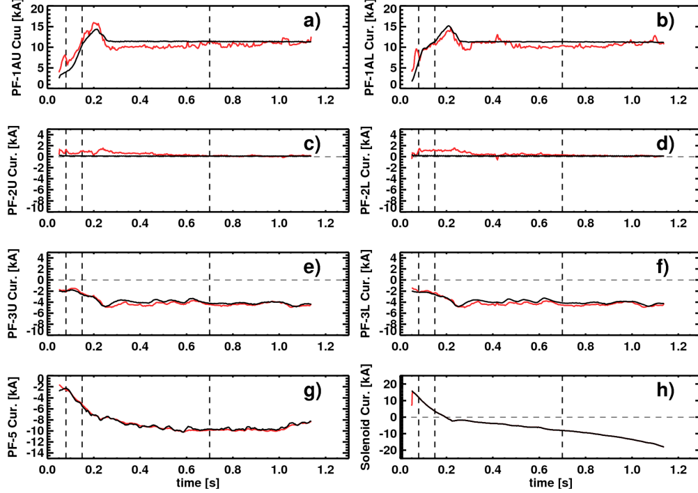
Fig. 4: Comparison of the actual and computed coil currents. The locations of the various coils are indicated in Fig. 3, and the dashed vertical lines correspond to the times in Fig. 3. See text for additional details.
