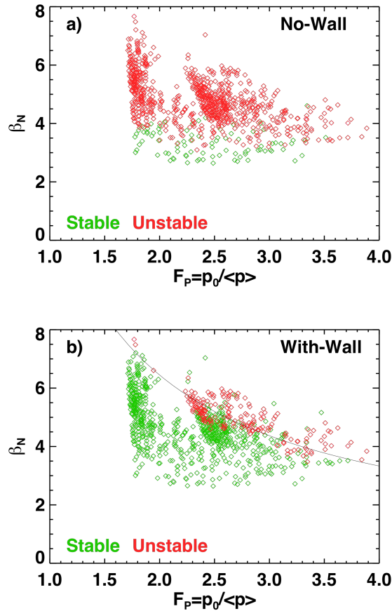
Fig. 35: Plots of the normalized- \beta vs. total pressure peaking factor. The colors are indicative of the n=1 ideal stability, without a wall in a) and with an ideally conducting wall at the location of the passive plates in b).
