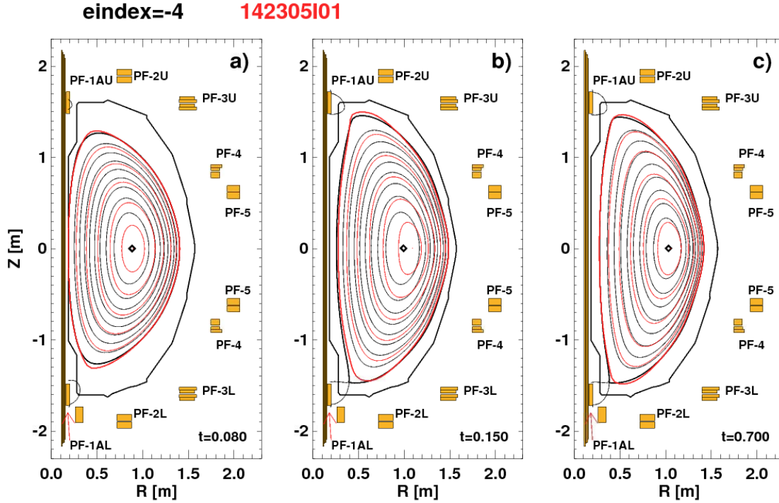
Fig. 3: Comparison of the input and calculated equilibria using free-boundary TRANSP. See the text for additional details.
