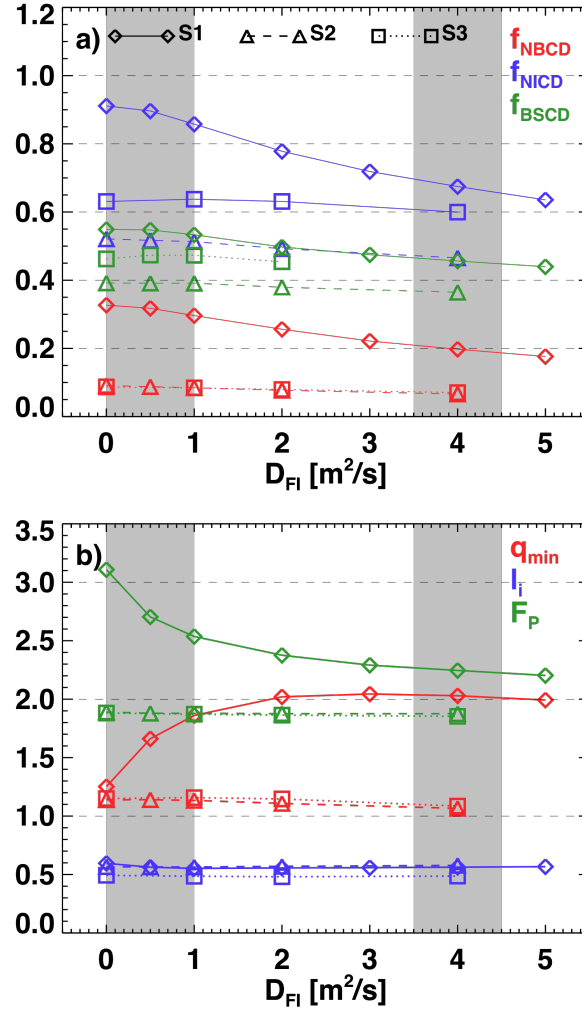
Fig. 11: Various parameters as a function of the spatially and temporally constant fast ion diffusion coefficient. The diamonds are for the S1 scenario with B_T=1T , I_P=1 MA and f_{GW}=0.72 , the triangles for the S2 scenario with 1.2 MA , 0.55 T and f_{GW}=0.86 , and the squares for the S3 scenario with 1.6 MA , 1.0 T , and f_{GW}=0.72 . See text for additional details.
