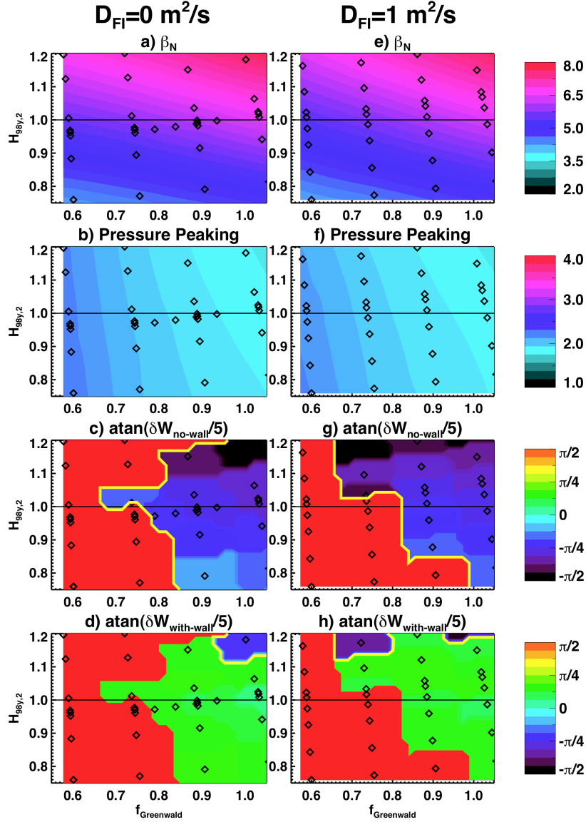
Fig 25: Ideal stability parameters for configurations in Fig. 24. See text for further details.
