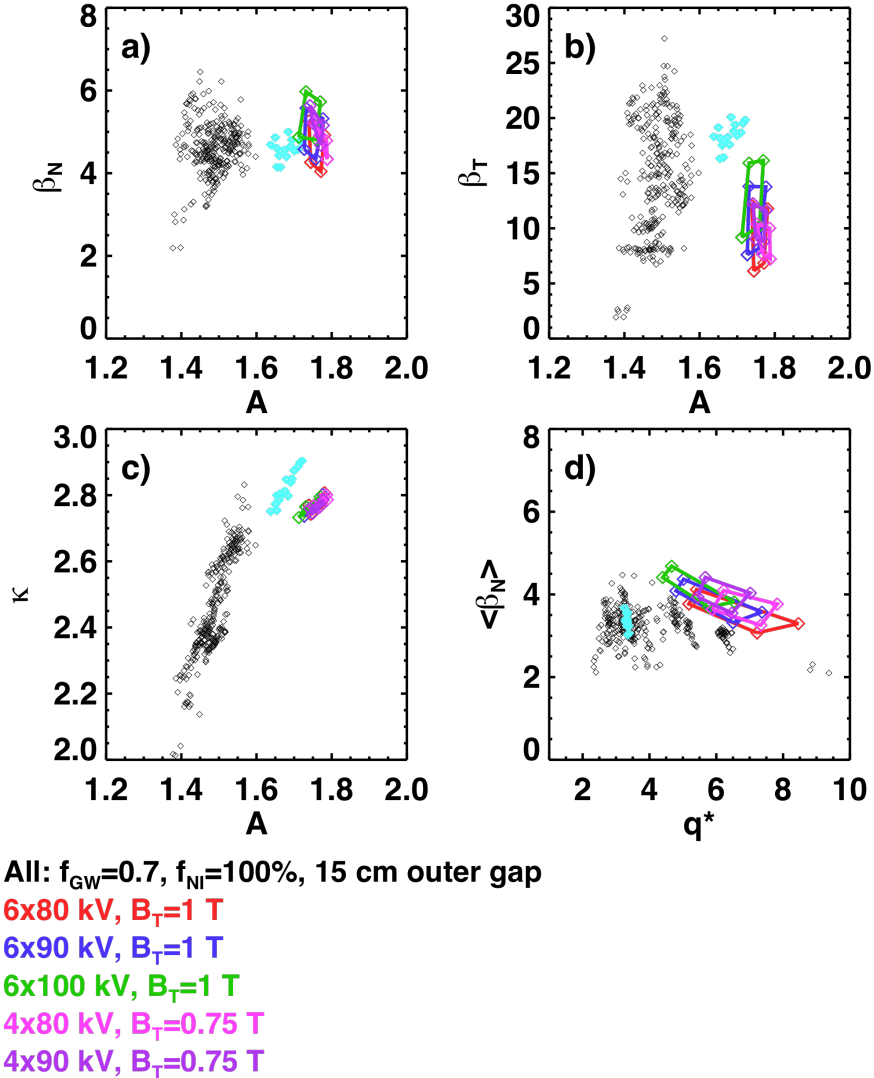
Fig. 31: Comparison of stability-related parameters between 100 % non-inductive scenarios for NSTX-Upgrade and achieved NSTX scenarios.
