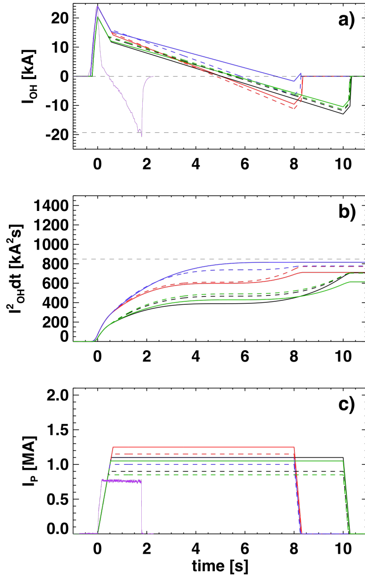
Fig 23: a) Model solenoid current, b) \int I_{OH}^2 dt , and c) plasma current evolution for the scenarios in Fig. 22. Also shown in frame a) and c) are the solenoid and plasma currents for NSTX discharge 129125.
