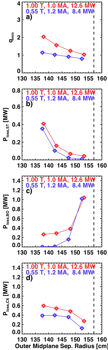
Fig. 8: Variation of the a) central safety factor, b) the shine-through power, c) the bad-orbit loss power, and d) the charge exchange loss power, as a function of the outer midplane separatrix radius, for the scans in Figs. 6 and 7. The radius of the outboard limiter is shown as a vertical dashed line.
