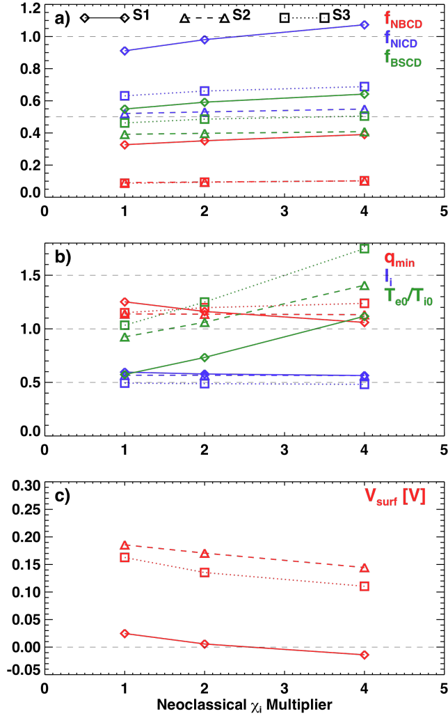
Fig. 14: Variation of selected quantities as a function of the multiplier on the ion neoclassical thermal diffusion coefficient, for fixed overall confinement. The symbols and linetypes correspond to the same discharge scenarios as in Fig. 11 and are explained in detail in Table 1. See text for additional details.
