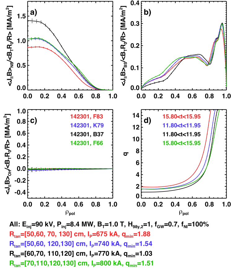
Fig. 28: Variation of the safety factor profile with various beam tangency radii, for 100 % non-inductive scenarios at B_T=1.0 T. The plasma current is allowed to vary in order to maintain the non-inductive state.
