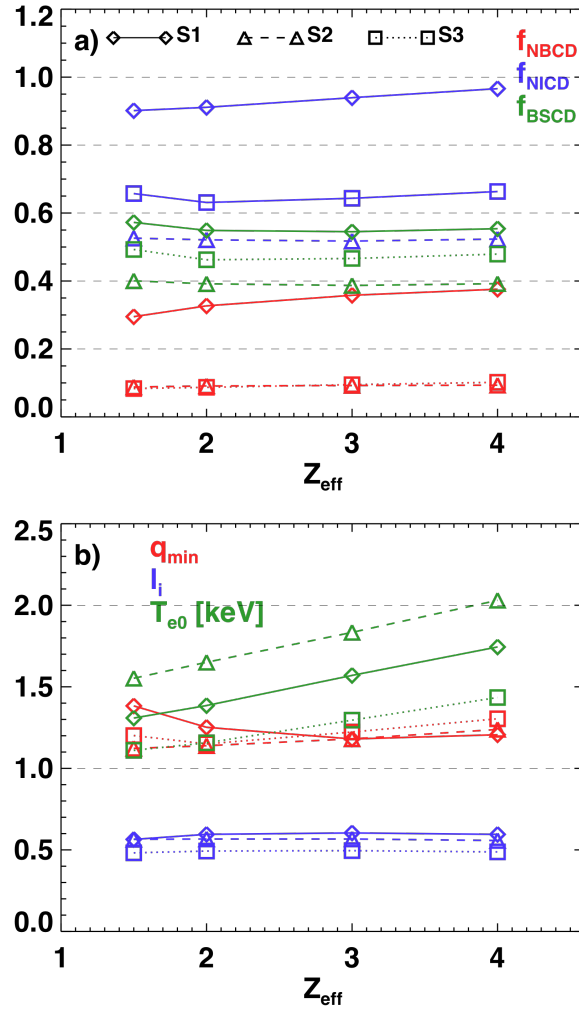
Fig. 15: Variation of selected quantities as a function of Z_{\text{eff}} , for fixed global confinement given by H_{98y,2}=1 . The symbols and linetypes correspond to the same discharge scenarios as in Fig. 11 and are explained in detail in Table 1. See text for additional details.
