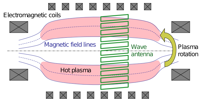
FIG. 3. A diagram of a mirror driven with waves. The wave antenna is a stationary magnetic ripple that produces rotation by interacting with alpha particles.
