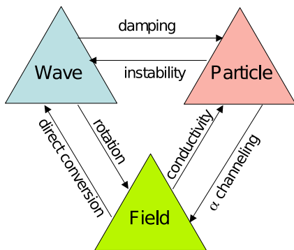
FIG. 1. Energy transfer between the wave, particle, and field energy. Applications or descriptions of each type are written by the arrows.
