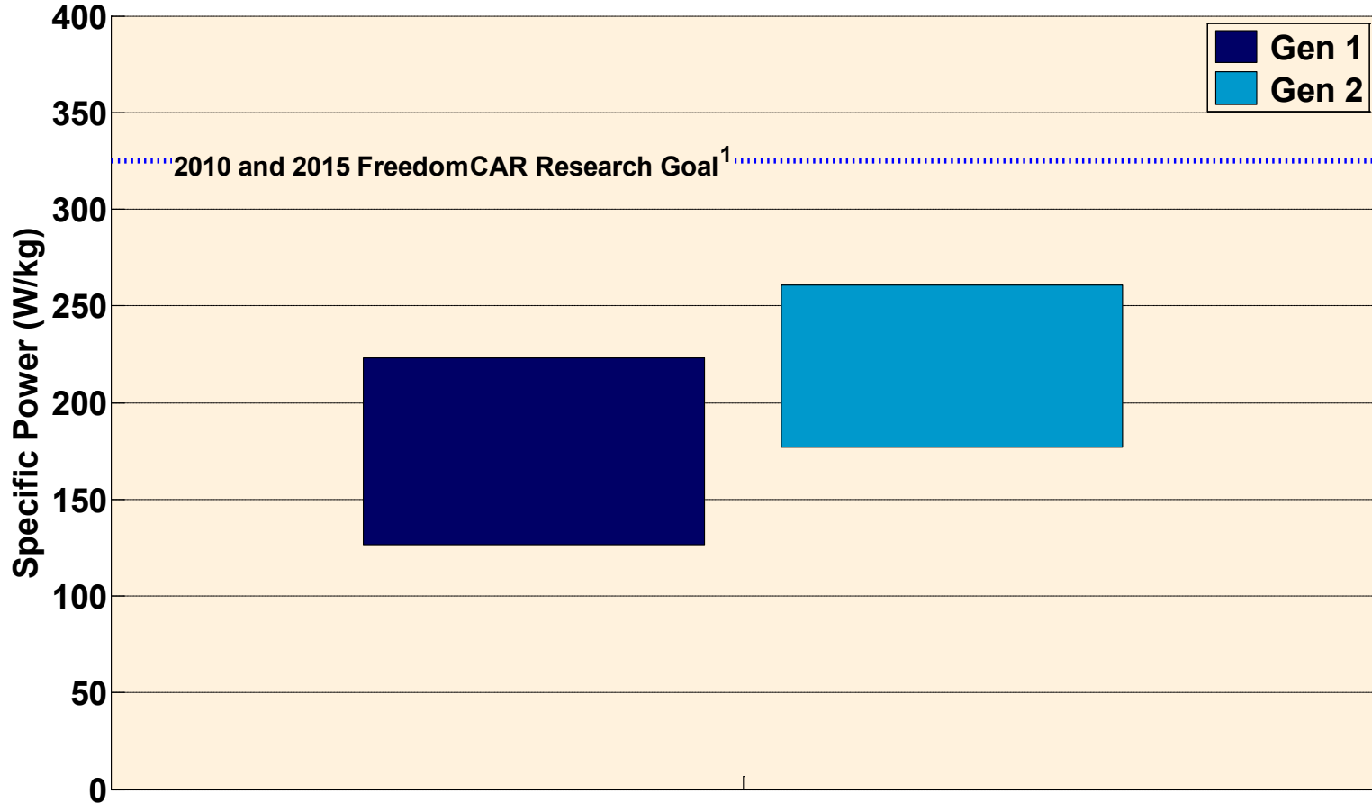
FC System (Including Hydrogen Storage) Specific Power (W/kg)
