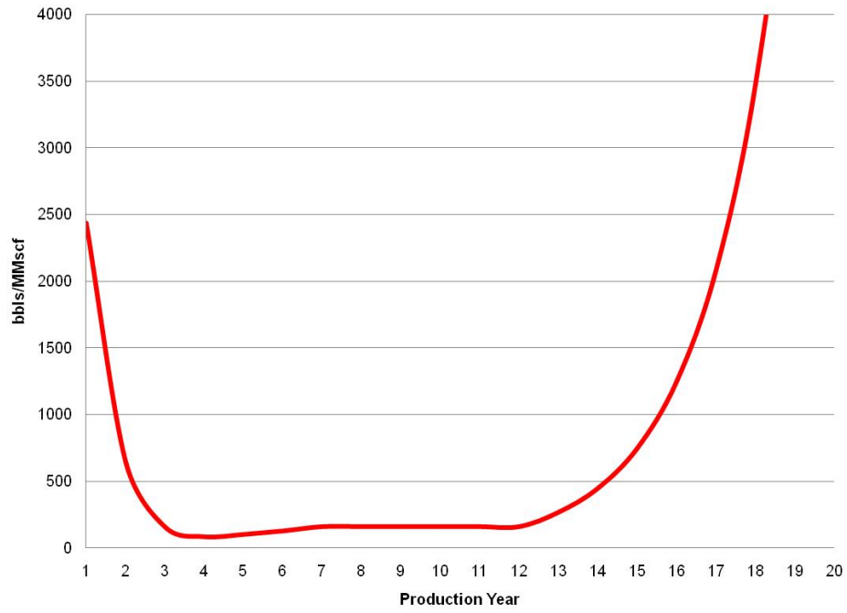
Figure 22 - Gas Water Ratio (bbls/MMscf) for Offshore Gas Hydrate Study
