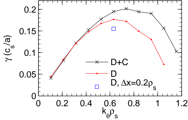
Fig. 1. (color online) Linear growth rate spectra at r/a=0.6 using deuterium and carbon and deuterium only. Also shown is the linear growth rate of the n=30 ( k_{\theta}\rho_s=0.63 ) mode using the exact same grid parameters as the non-linear simulations below ( L_x=80\rho_s , n_x=400 , \Delta x=0.2\rho_s ).
