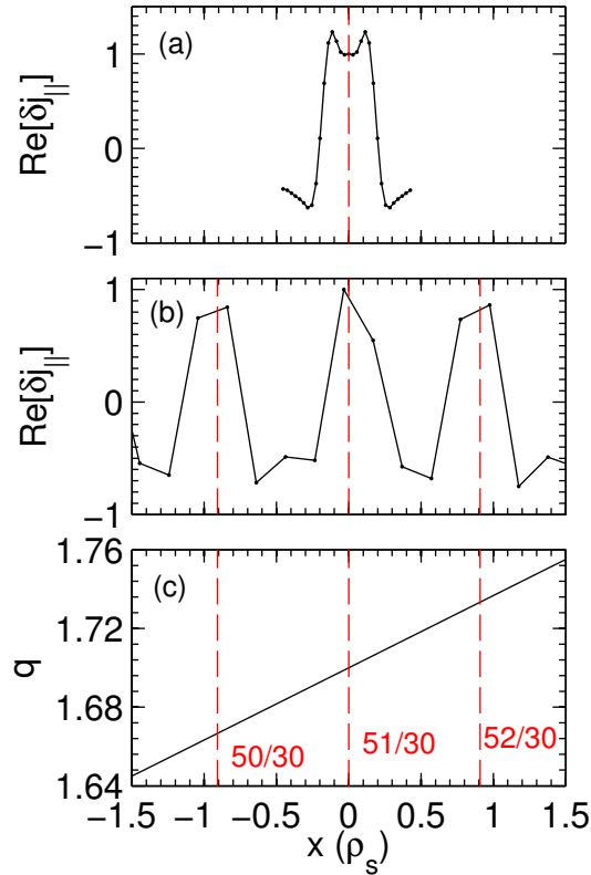
Fig. 2. (color online) Radial variation of parallel current perturbations from linear simulations at \theta=0 for two different perpendicular resolutions: (a) \Delta x=0.03 \rho_s ( L_x=0.9 \rho_s , n_x=32 ) (typical flux-tube domain), (b) \Delta x=0.2 \rho_s ( L_x=80 \rho_s , n_x=400 ) (similar domain as non-linear simulations). (c) The q profile used in each simulation. Dashed lines are located at each rational surface associated with the n=30 ( k_{\theta}\rho_s=0.63 ) mode.
