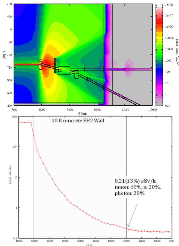
Figure 7. Total dose with a 40 cm iron safety collimator and 3 m concrete EH2 wall: 2D distribution on beam height and 1D on the primary incident direction.
