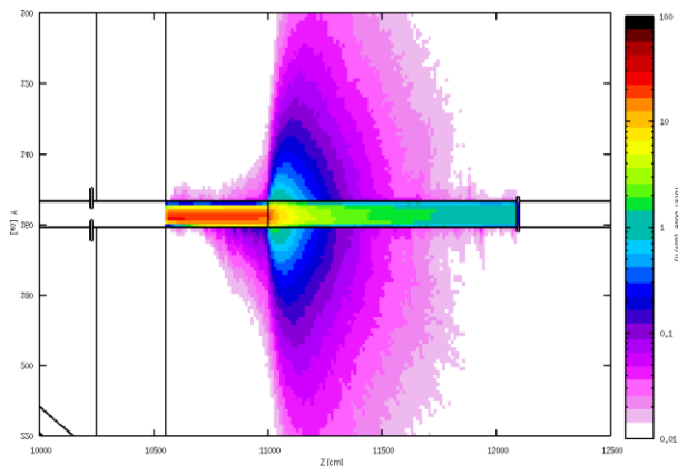
Figure 8. Total dose in EH2 due to radiation leakage from beam pipe.
