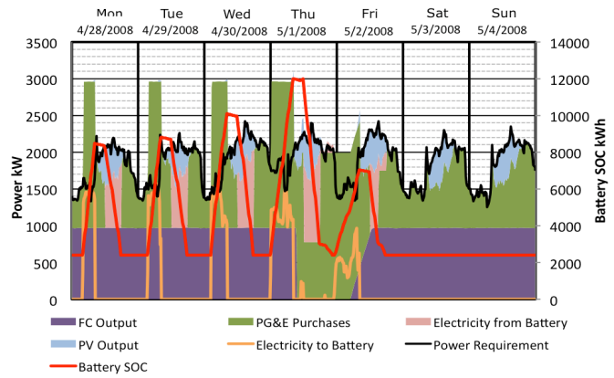
Fig. 4 Optimized May 2008 Week NaS Battery Operation Notice that the battery is left discharged over the weekend. Round-trip losses are significant for NaS batteries, and 30% is the average here. In general, the battery is charged in the early morning hours and discharged during the following afternoon. Strangely the state-of-charge is considerably lower during a fuel cell outage, a surprising result driven by the off peak demand charges.
