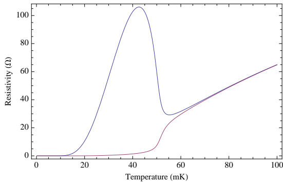
FIG. 3: In-plane field rounded longitudinal resistivities \rho_{x,x,yy} along the easy x-axis (red) and hard y-axis (blue) obtained from the conductivities in (19) are plotted versus temperature. A mean field crossover function has been used in the expression for the resistivities.
