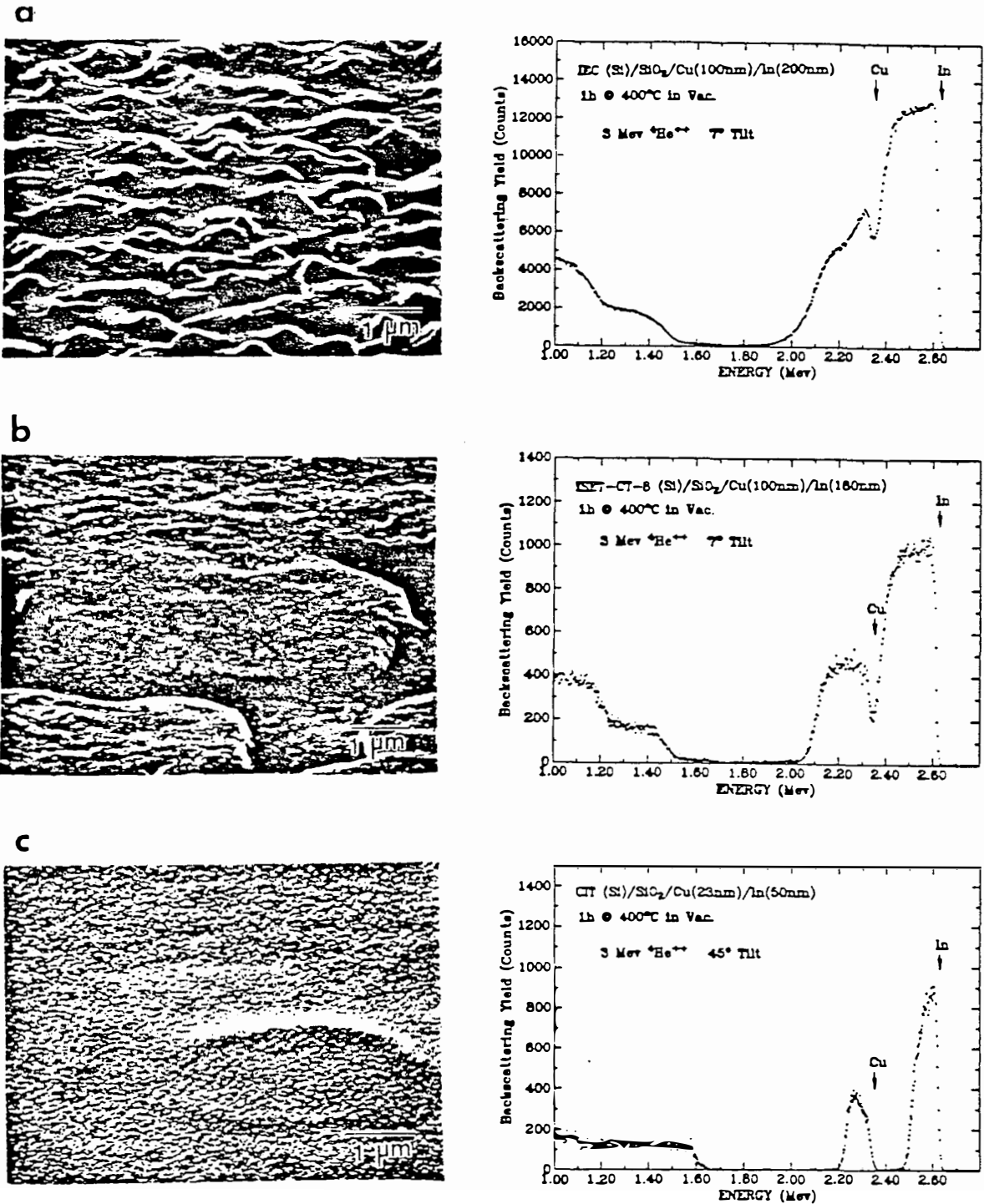
Fig. 6 Scanning electron micrographs and 3 MeV 4 He ++ backscattering spectra of Cu/In bilayers after annealing for 1 h at 400°C, in vacuum, deposited by (a) e-beam evaporation of both layers (b) e-beam evaporation of Cu and electrodeposition of In (c) rf sputtering of both layers.
