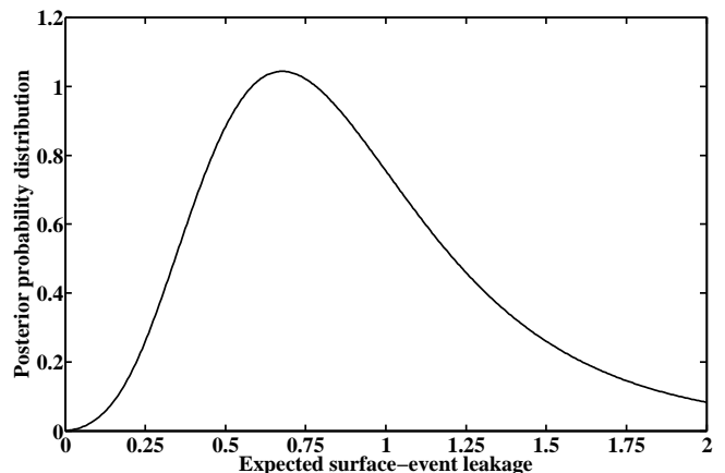
FIG. 4. Distribution of the surface-event leakage estimate in the 25-150 \text{ keV} energy range. See text for details.
