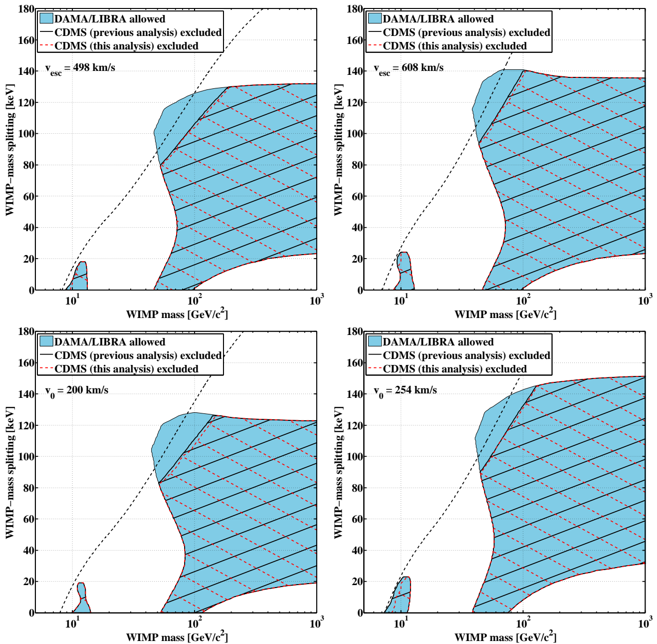
FIG. 10. (color online). Constraints from CDMS on the iDM parameter space allowed by DAMA/LIBRA. Same as Fig. 9 but with different velocity-distribution parameters, as given in the plots. All other parameters remain unchanged.
