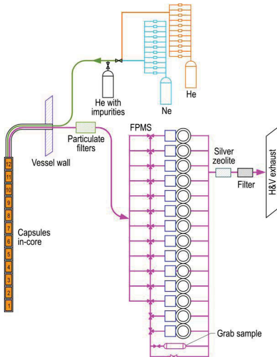
Fig. 5: AGR experiment gas flow path
