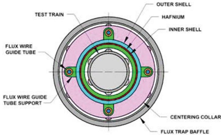
Fig. 4: AGR-3/4 irradiation housing cross-section
