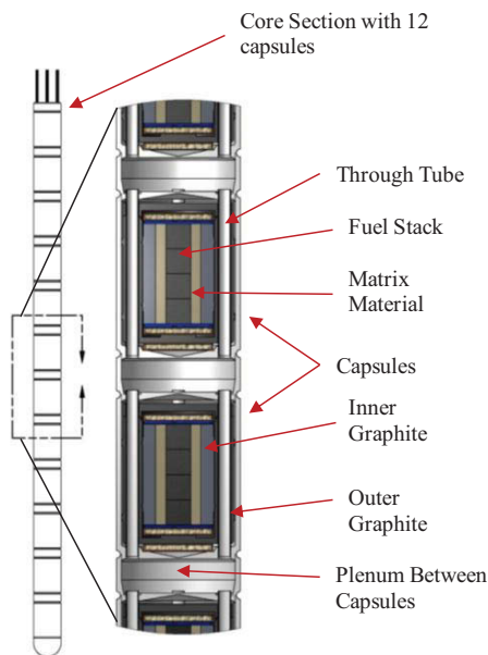
Fig. 3: AGR-3/4 test train vertical section
