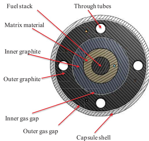
Fig. 2: AGR-3/4 capsule cross-section
