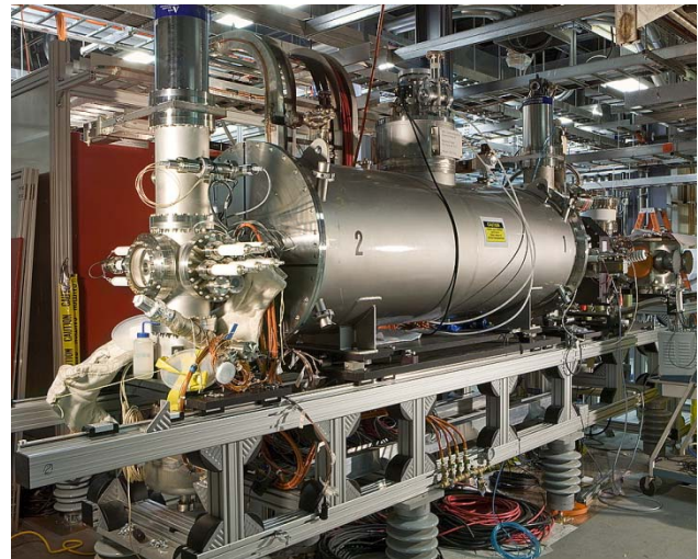
Fig 3: Photo of the EBIS.
