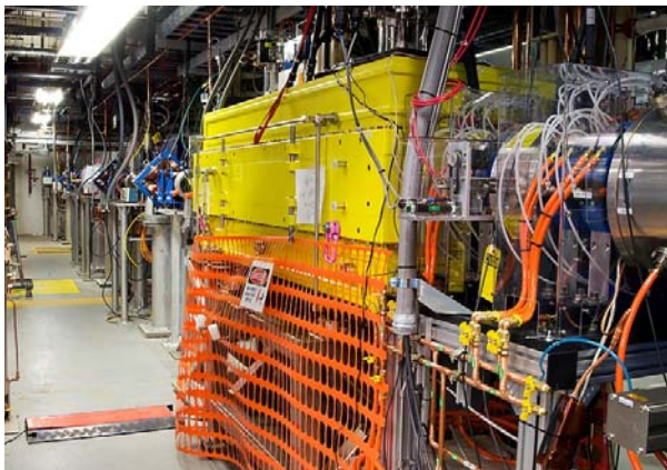
Fig. 5: Looking down the HEBT line.
