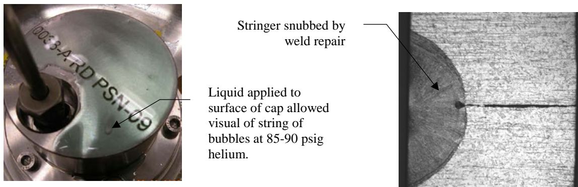
Figure 4 Surface Inspection and Metallographic Cross Section of Leak
