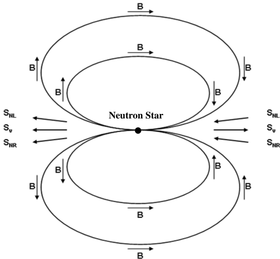
Figure 1. Schematic diagram of the magnetic fields, \underline{B} , surrounding a nascent neutron star and the spins of the ^{14}\text{N} nuclei, S_N , and of the neutrinos, S_\nu , emitted from the supernova that created the neutron star.
