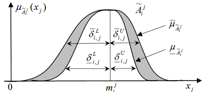
Fig. 3 Illustration of the non-symmetric IT2 input Gaussian fuzzy set \tilde{A}_i^j .
