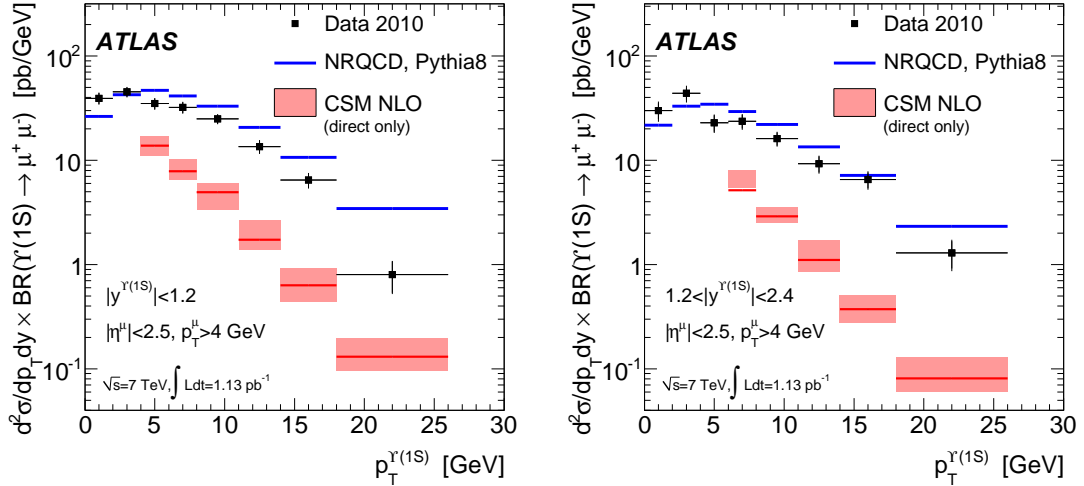
Figure 3: The differential \Upsilon(1S) cross-section for the |y^{\Upsilon(1S)}| < 1.2 (left) and 1.2 < |y^{\Upsilon(1S)}| < 2.4 (right) as function of p_T^{\Upsilon(1S)} for p_T^\mu > 4 GeV and |\eta^\mu| < 2.5 on both muons. Also shown is the colour-singlet NLO (CSM) prediction using m_T for the renormalisation and factorisation scales. The shaded area shows the change in the theoretical prediction when varying the renormalisation and factorisation scales by a factor of two. The CSM NLO calculation accounts only for direct production of \Upsilon(1S) mesons and not for any feed-down from excited states. The NRQCD prediction as implemented in PYTHIA8 is also shown for a particular choice of parameters as discussed in the text.
