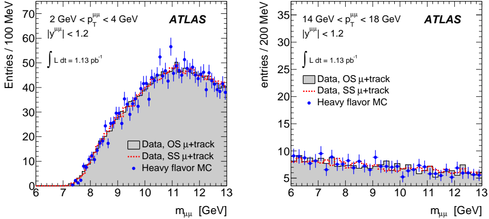
Figure 2: Two examples of the templates used for the description of the dimuon mass dependence of the background are shown. The solid histogram shows the opposite-sign (OS) \mu +track, the dashed histogram shows the same-sign (SS) \mu +track and the filled circles show the histogram derived from dimuon events in open b\bar{b} and c\bar{c} MC (heavy flavour MC). The error bars reflect the statistical uncertainty on the MC-based template. All histograms are normalised to the same absolute amount of background as determined in the fit for each kinematic bin (see also Fig. 1 and Section 6).
