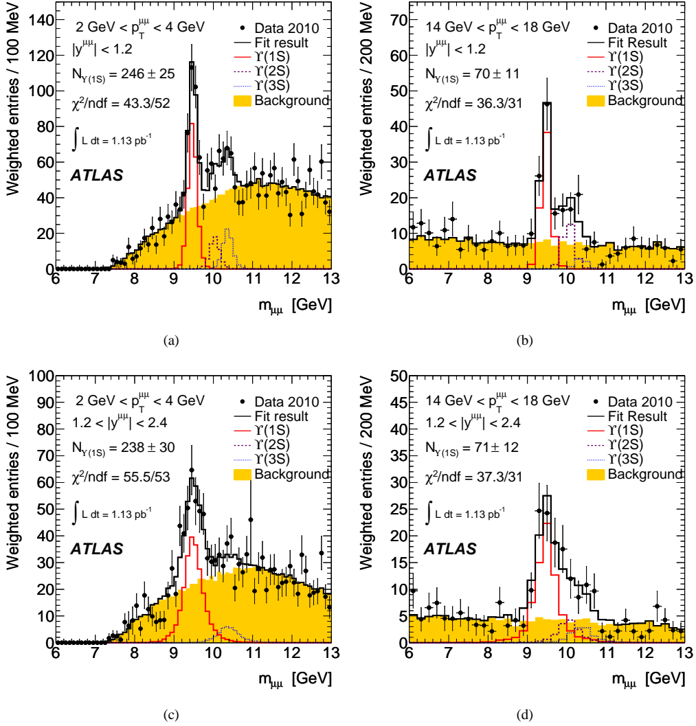
Figure 1: Dimuon mass distributions for four representative bins in y^{\mu\mu} and p_T^{\mu\mu} . The data (filled circles) are shown together with the result of the unbinned maximum likelihood fit (histogram) as explained in the text. The shaded histogram shows the background contribution, and the three other histograms show the contributions from the three \Upsilon states. All histograms are normalised by the factor determined in the fit. In the individual plots, the fitted N_{\Upsilon(1S)} yield with its statistical uncertainty, the \chi^2 and the number of degrees of freedom are also given. It should be noted that this is simply a binned graphical representation of the fit; the actual fit is unbinned and interpolates the template histograms to obtain the input probability density function.
