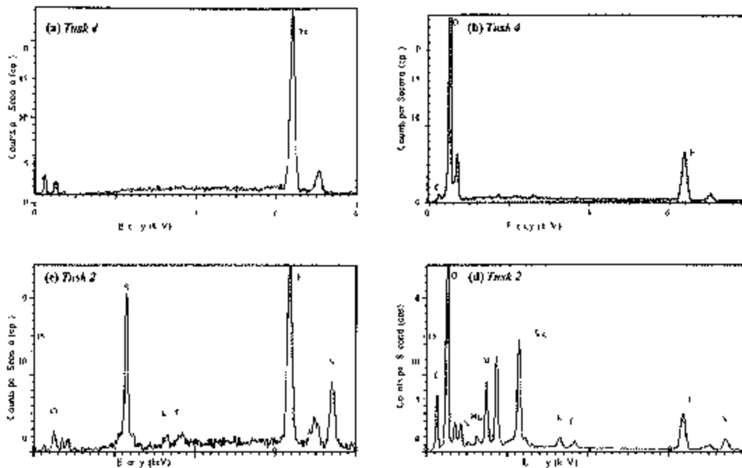
Fig 3 X-ray fluorescence (XRF) spectra showing the compositional variability within and between particles from two different tusks. Compositions range between native Fe (a), FeO (b), FeNiS (c, d). Silicate compositions in d are probably due to contamination from host sediments during burial.
