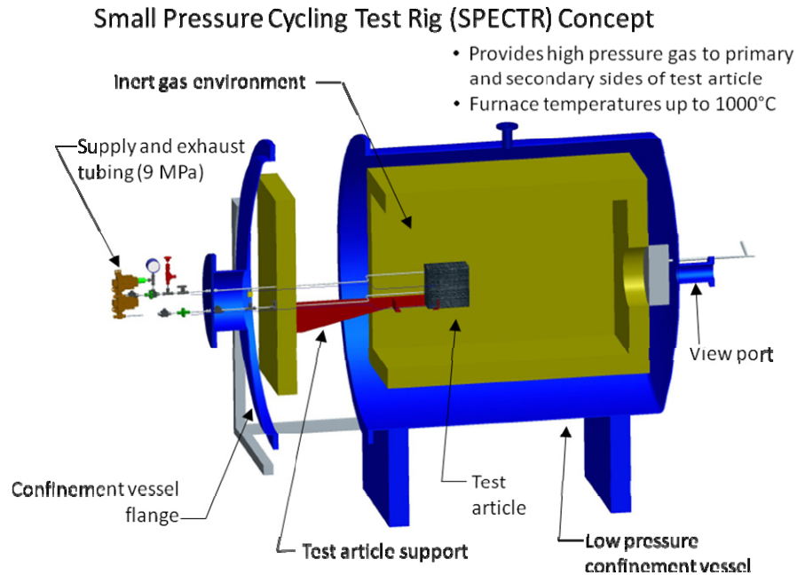
Figure E-9. The SPECTR test system at the INL.
