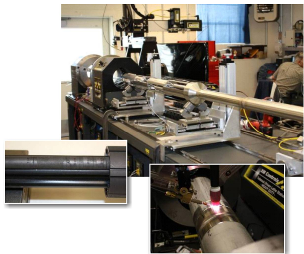
Figure D-9. Photographs of AGC-1 test train during assembly.
