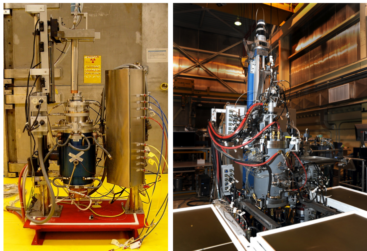
Figure D-5. Furnaces used in accident safety testing of TRISO fuel: (a) ORNL Core Conduction Cooldown Test Facility (b) INL Fuel Accident Condition Simulator.
