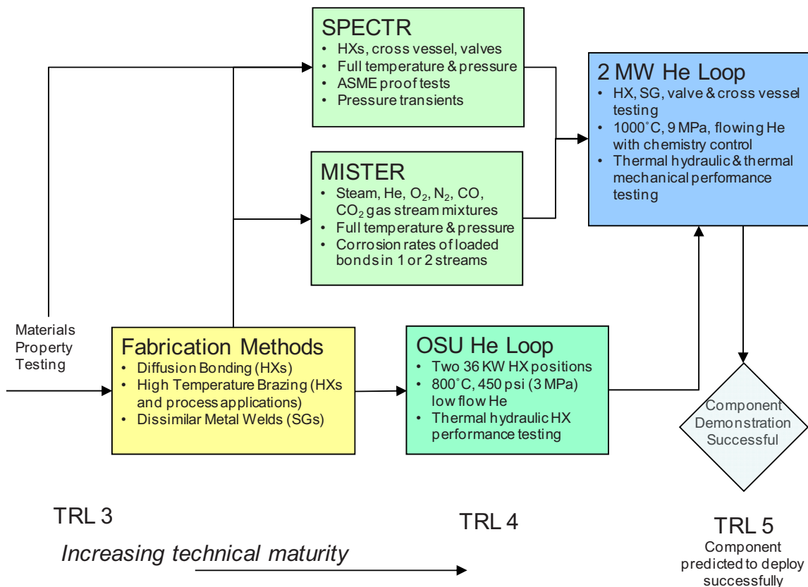
Figure E-10. Heat Transport Component Test Capability required to achieve TRL-5.
