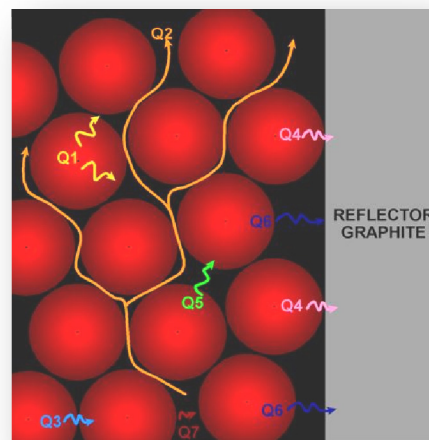
Figure D-12. Coupled heat transfer and fluid flow near the wall of a pebble bed reactor.
