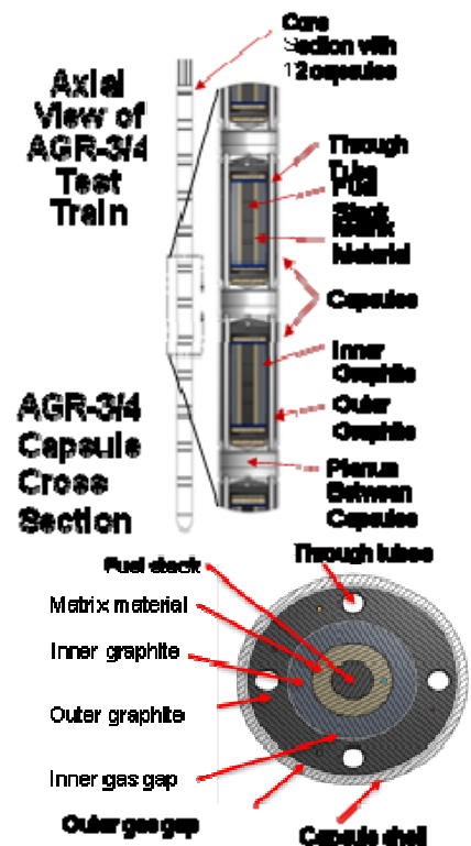
Figure K-3. AGR 3/4 capsule.
