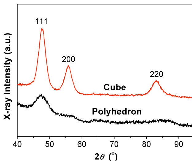
Figure 2. XRD patterns of Rh nanopolyhedra and nanocubes.
