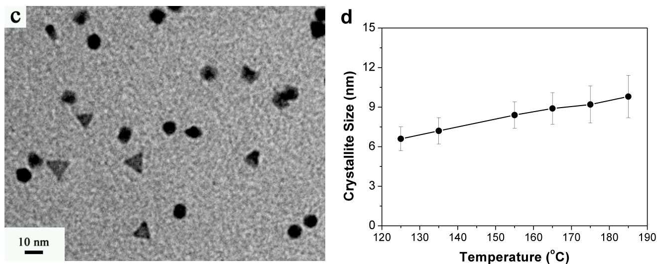
Figure 4. TEM images of Rh nanopolyhedra synthesized in 20 ml ethylene glycol under an Ar atmosphere at different temperatures for 2 h, using 2.5 mM [\text{Rh}(\text{Ac})_2]_2 and 100 mM PVP: (a) 125 °C; (b) 135 °C; (c) 165 °C. (d) Crystallite size of the Rh nanopolyhedra as a function of synthetic temperature.
