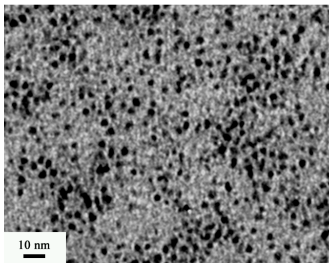
Figure 8. TEM image of Rh nanocrystals synthesized in 20 ml ethylene glycol under an Ar atmosphere at 165 °C for 1.5 h, using 2.5 mM [\text{Rh}(\text{Ac})_2]_2 , 5 mM TMAB, and 50 mM PVP.
