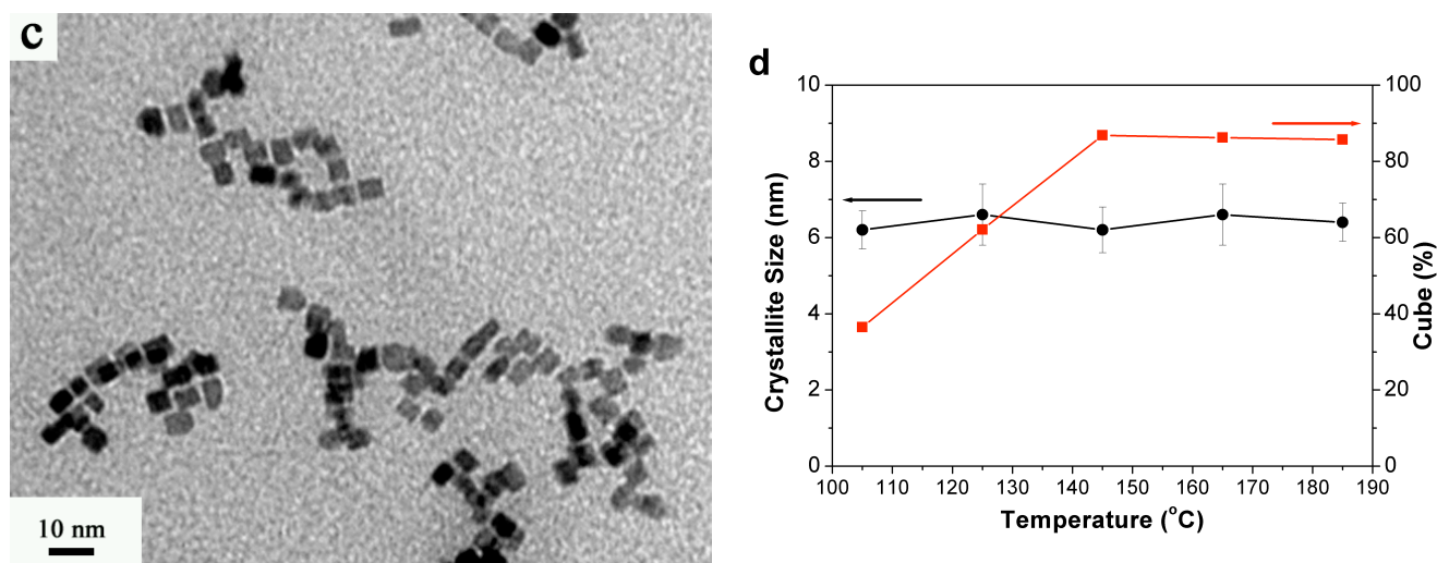
Figure 6. TEM images of Rh nanocubes synthesized in 20 ml ethylene glycol under an Ar atmosphere at different temperatures for 1.5 h, using 10 mM RhCl 3 , 50 mM TTAB and 200 mM PVP: (a) 105 °C; (b) 125 °C; (c) 145 °C. (d) Crystallite size of the Rh nanocubes as a function of synthetic temperature.
