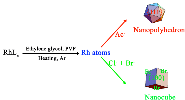
Figure 7. A schematic illustration of the reaction pathways responsible for the formation of (111) and (100)-oriented Rh nanocrystals.
