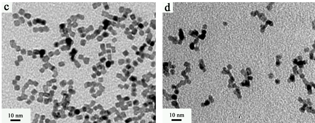
Figure 5. TEM images of Rh nanocrystals synthesized in 20 ml ethylene glycol under an Ar atmosphere at 185 °C for 1.5 h: (a) 10 mM RhCl 3 , 50 mM TEAB, 200 mM PVP; (b) 10 mM RhCl 3 , 50 mM TDAB, 200 mM PVP; (c) 10 mM RhCl 3 , 50 mM TTAB, 200 mM PVP; (d) 5 mM RhCl 3 , 25 mM TTAB, 100 mM PVP.
