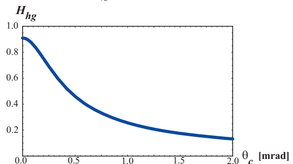
Figure 1: Geometric loss factor H_{\text{hg}} vs. crossing angle.
