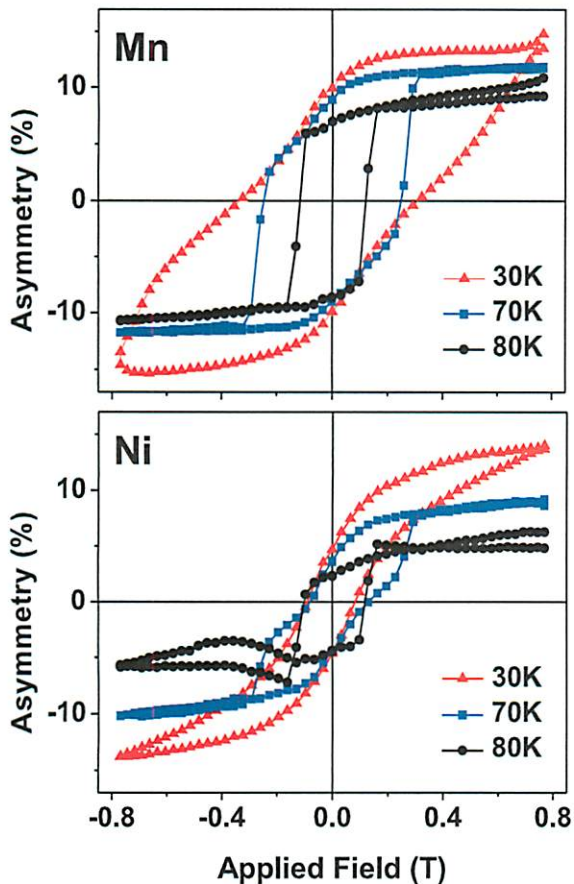
FIG. 10: (Color Online) Mn and Ni XMCD hysteresis loops as a function of temperature for the annealed ( \text{Mn}_{\text{Oh}}^{4+} -rich) NMO film.
