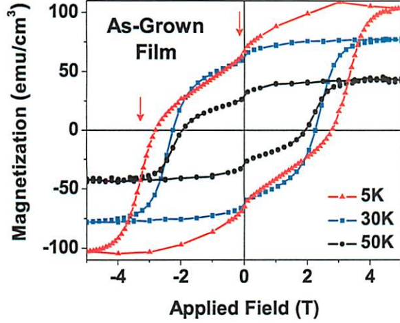
FIG. 7: (Color Online) SQUID hysteresis loops of as-grown ( \text{Mn}_{\text{O}_h}^{4+} -poor) NMO film at various temperatures, showing large coercive fields and double transition hysteresis loops (marked by arrows) for all temperatures.
