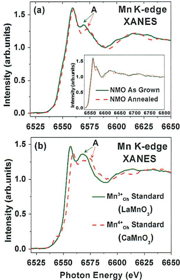
FIG. 3: (Color Online) Mn XANES. (a) Comparison between as-grown and annealed films with feature A marked by arrows. Inset is extended energy range view. (b) Mn valence specific standards illustrating that both absorption edge and feature A shift to higher energy for increasing Mn valence.
