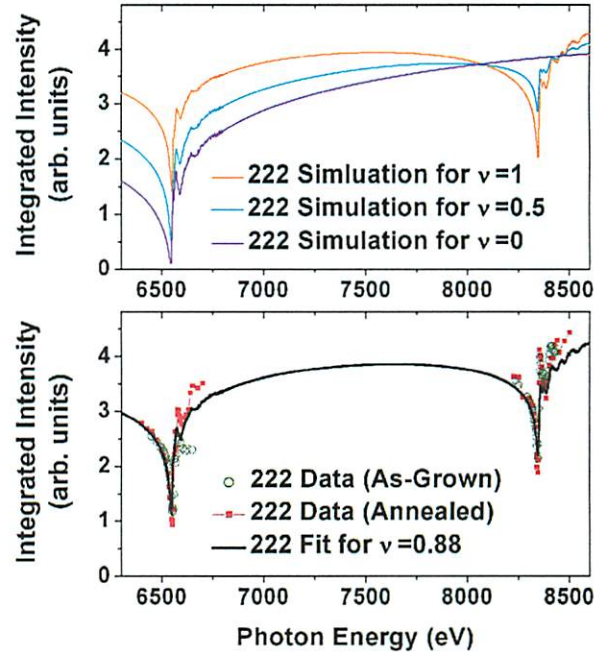
FIG. 4: (Color Online) Anomalous X-ray scattering of NMO 222 reflection. (a) Simulations with inversion parameters \nu = 0, 0.5, 1 . (b) Data from as-grown and annealed films with nonlinear least square fit of \nu = 0.88 .
