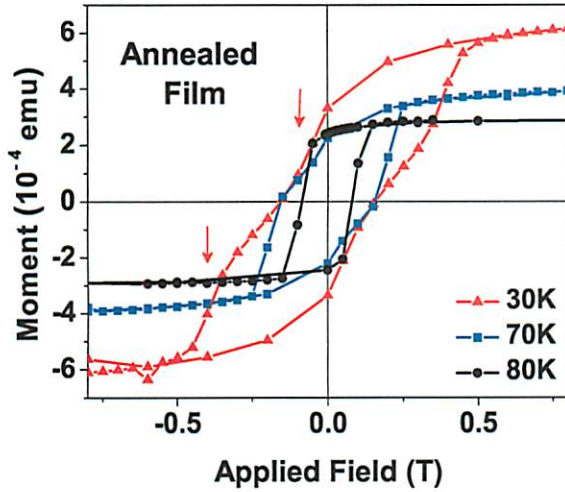
FIG. 8: (Color Online) SQUID hysteresis loops of an annealed ( \text{Mn}_{\text{O}_h}^{4+} -rich) NMO film at various temperatures, showing single and double (arrows) transition hysteresis loops at high and low temperatures, respectively.
