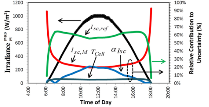
Fig. 2. Calculated POA irradiance for PV reference device, along with accompanying expanded uncertainty error bars (left axis), and relative contributions to total uncertainty from the inputs to Eq. (4).
