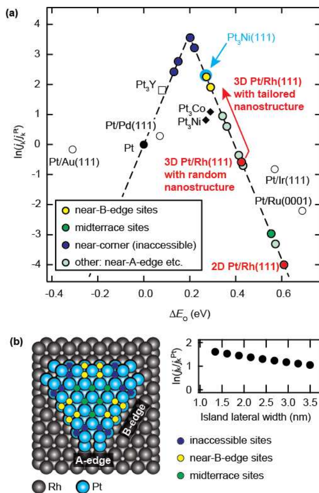
Figure 7. (a) Predicted individual ORR activities of individual fcc threefold hollow sites on 3D Pt/Rh(111). For comparison, measured ORR activities are shown for a range of bimetallic electrocatalysts 5,8,24 including the previous measurement on 3D Pt/Rh(111). 24 The latter can be considered to represent a weighted average of the individual site contributions plotted with light green, dark green and yellow markers. (b) Bilayer islands with maximized occurrence of near-B-edge sites (yellow). The graph shows the ORR activity enhancement for a series of such islands whose lateral width is varied by changing the length of the B-edges while the A-edges are fixed at 0.54 nm length.
