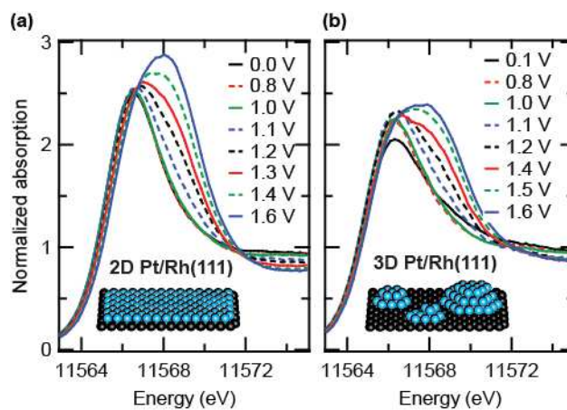
Figure 2. In situ Pt L_3 HERFD XAS for 1 ML Pt/Rh(111) in 0.01 M HClO_4 : (a) 2D Pt film, (b) 3D Pt islands. Spectra were recorded in the order of increasing electrochemical potentials.
