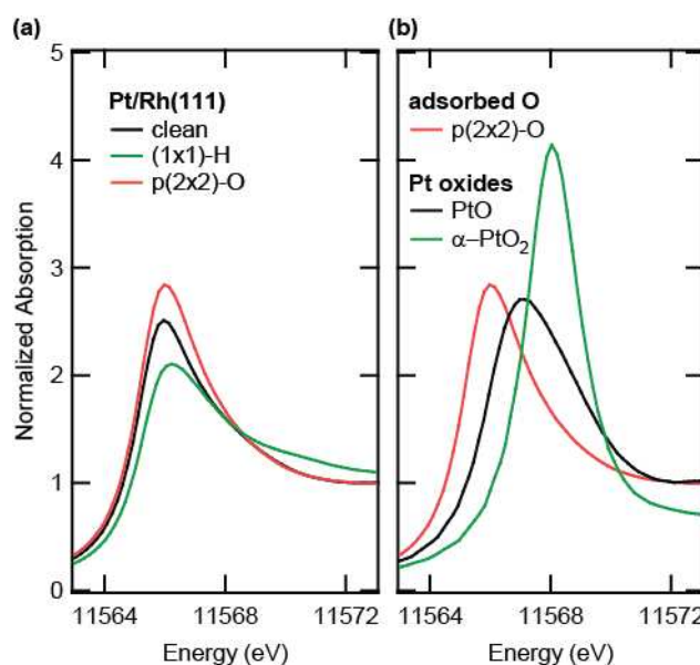
Figure 3. Calculated HERFD XAS, using the FEFF8 code, for clean, H_{ad} - and O_{ad} -covered Pt/Rh(111).
