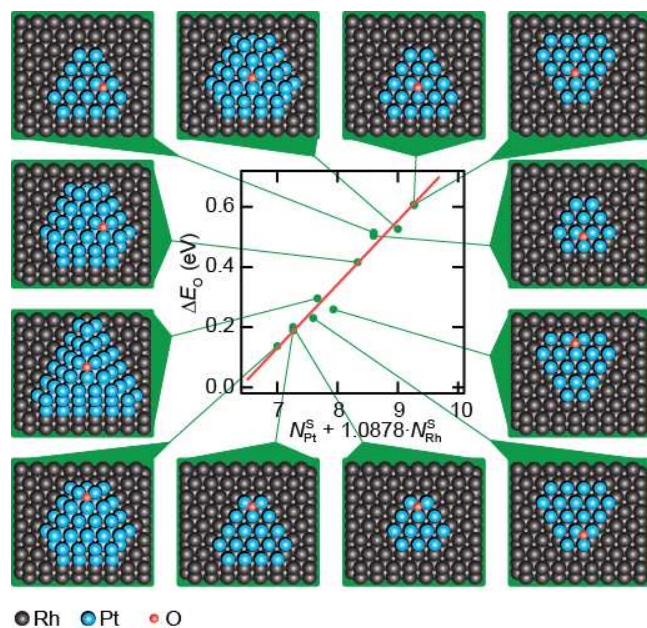
Figure 6. DFT calculations of the adsorption energy \Delta E_{\text{O}} of a single O atom on Pt/Rh(111) model structures, shown as relative values compared to Pt(111) ( \Delta E_{\text{O,Pt(111)}} = 0 ). The corresponding adsorption energy for each structure is plotted as a function of the effective coordination number around the O adsorption site, and a linear fit (red line) is shown. The linear relationship can be used to estimate \Delta E_{\text{O}} for any other fcc threefold hollow site on Pt islands with various shapes and sizes.
