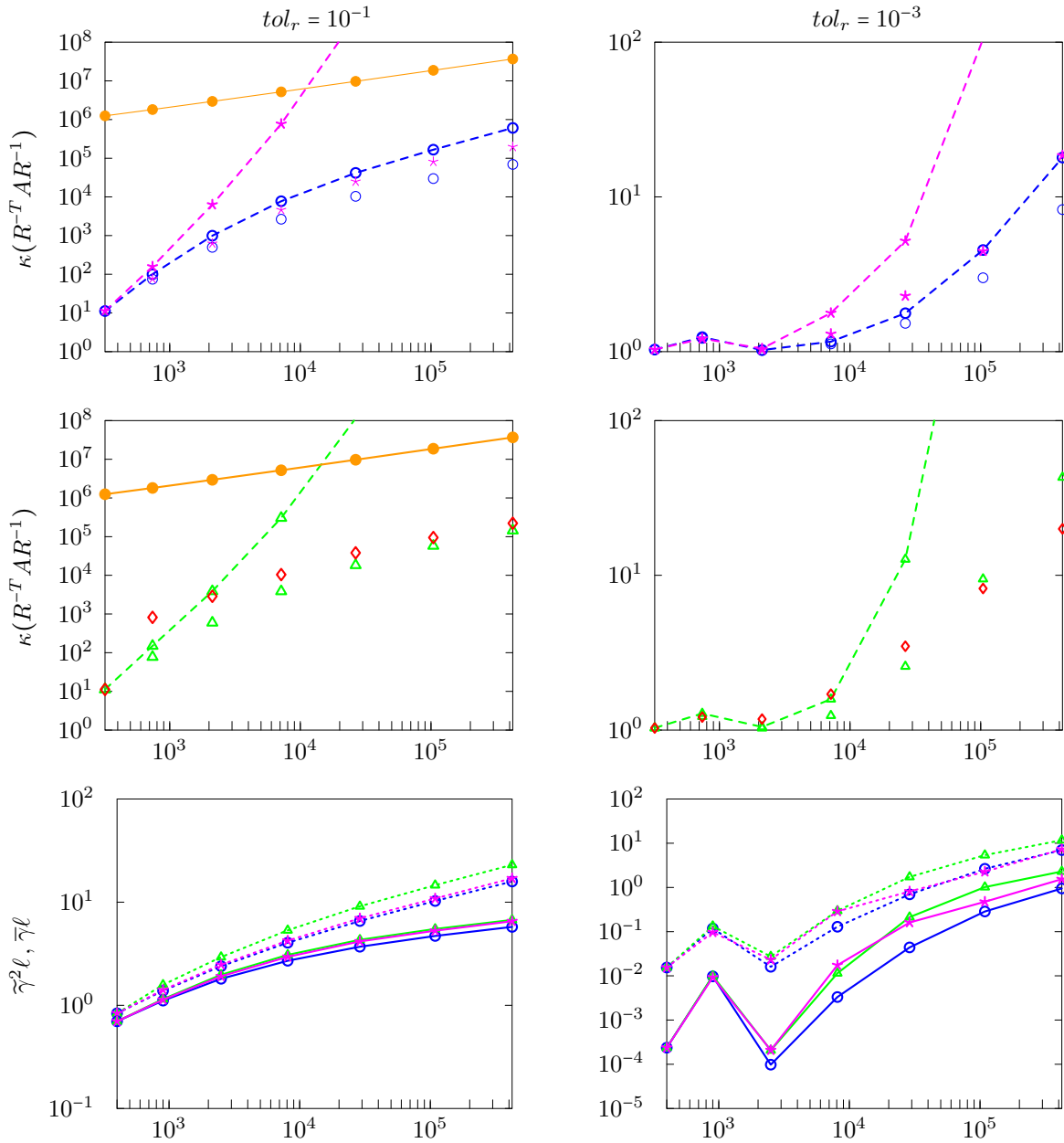
Figure 4: Condition number \kappa(R^{-T}AR^{-1}) for various strategies and the related upper bounds (top and middle), together with the corresponding accuracy parameters \bar{\gamma}\ell, \bar{\gamma}^2\ell (bottom) for truncation threshold tol_r set to 10^{-1} (left) and 10^{-3} (right) and for different values of N^2 . Markers \circ (blue) corresponds to one-level variant, \star (magenta) to SSS, \triangle (green) to HSS, and \diamond (red) to [27]. On the top and middle plots, isolated markers correspond to \kappa(B^{-1}A) , dashed lines connect their upper bounds and \bullet (orange) connected by a solid line represent \kappa(A) . On the bottom plots, dotted lines depict \bar{\gamma}\ell (see Corollary 3.4) and solid ones stand for \bar{\gamma}^2\ell (see Corollary 3.6).
