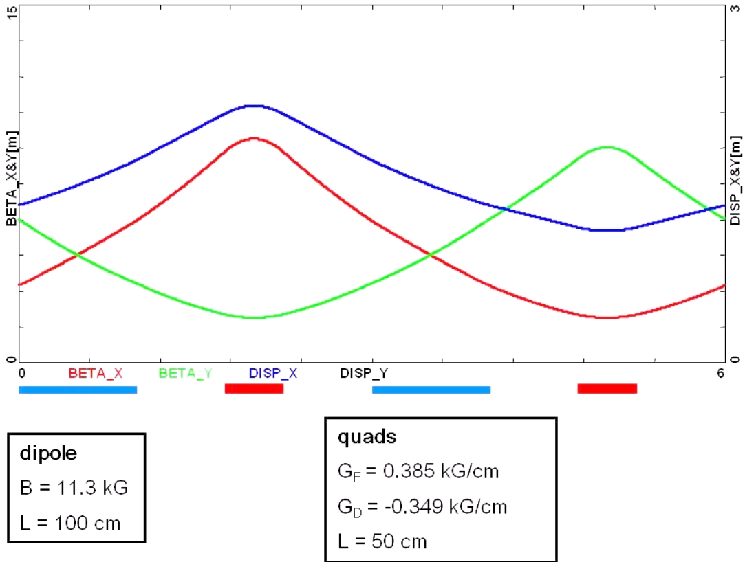
Figure 48. Periodic 90^\circ FODO 6 m inward-bending cell, including a pair of rectangular bends interleaved between quads. All elements are equally spaced.
