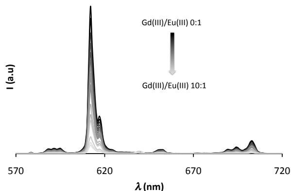
Fig. 4 Spectrofluorimetric competition titration of [\text{Eu}^{\text{III}}(3,4,3\text{-LI}(1,2\text{-HOPO}))]^- against Gd(III). [\text{Eu}^{\text{III}}] = [\text{3,4,3-LI}(1,2\text{-HOPO})] = 5 \text{ } \mu\text{M} , [\text{Gd}^{\text{III}}] = 0.05 \text{ mM} , 0.1 \text{ M KCl} , 0.1 \text{ M HEPES} , \text{pH} = 7.4 , 25.0 \text{ }^\circ\text{C} , \lambda_{\text{exc}} = 325 \text{ nm} . The luminescence signal resulting from the sensitization of \text{Eu}^{\text{III}} by 3,4,3-LI(1,2-HOPO) decreases while the \text{Gd}^{\text{III}} concentration increases
