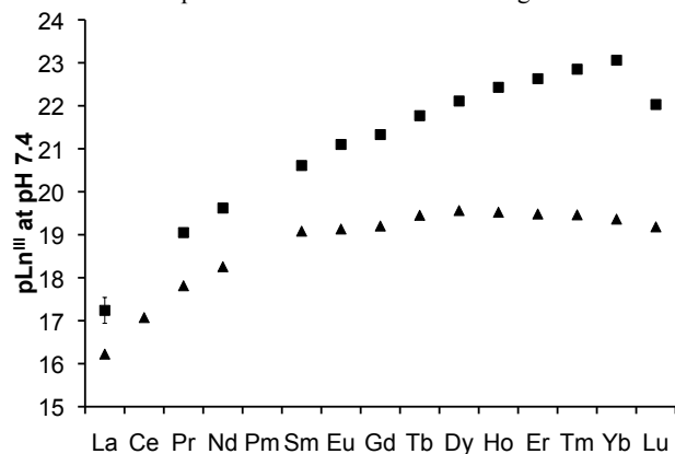
Fig. 5 Comparison of the pM values obtained for the Ln III complexes of 3,4,3-LI(1,2-HOPO) (■) and DTPA 16 (▲).
