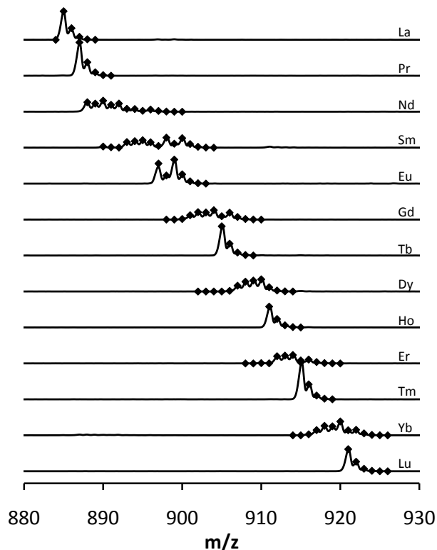
Fig. 6 Mass spectra of 50 \mu\text{M} [\text{Ln}^{\text{III}}(3,4,3\text{LI}(1,2\text{-HOPO}))]^- solutions directly injected in the ESI-MS at pH = 7.4 (solid lines). The diamonds represent the theoretical calculated isotope patterns for the complexes.
