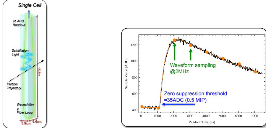
(b) The response from each detection cell is amplified and shaped by a custom ASIC and then sparsely sampled by a waveform digitizer.
