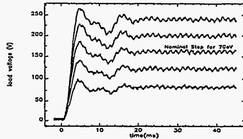
Figure 3: Step Response Family of Quadrupole Power Supply
