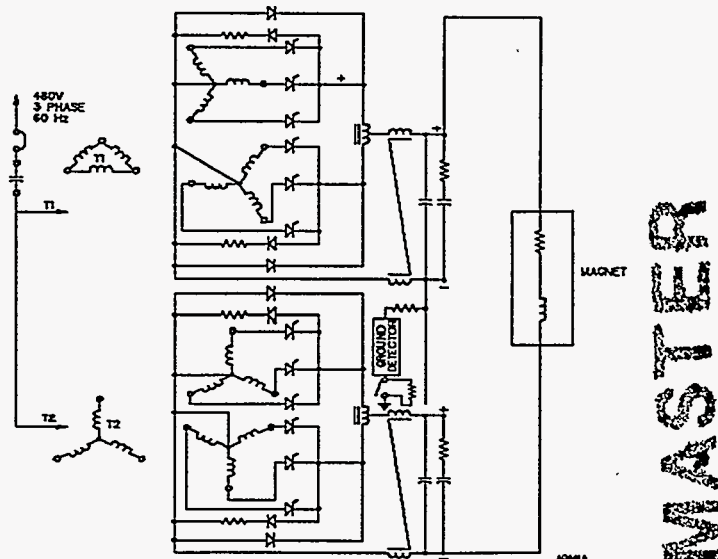
Figure 1: Simplified Schematic of Quadrupole Power Supply
