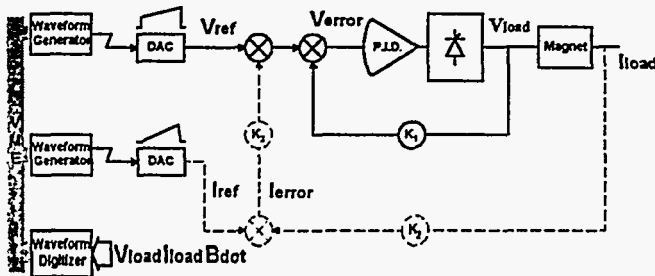
Figure 2: Control Scheme Block Diagram
