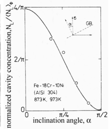
Figure 3. Creep cavity density as f_n (GB orientation) with respect to the loading axis [7].
