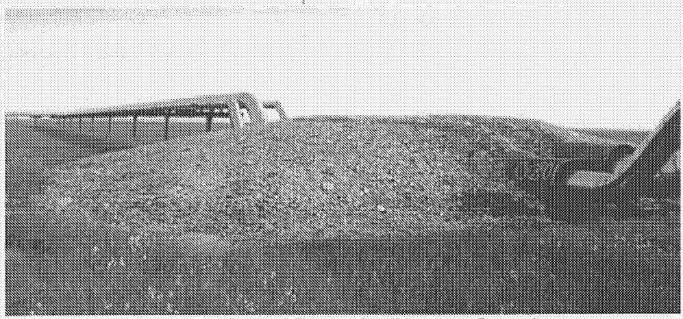
Figure 8. Gravel Ramp for Pipeline Crossing
