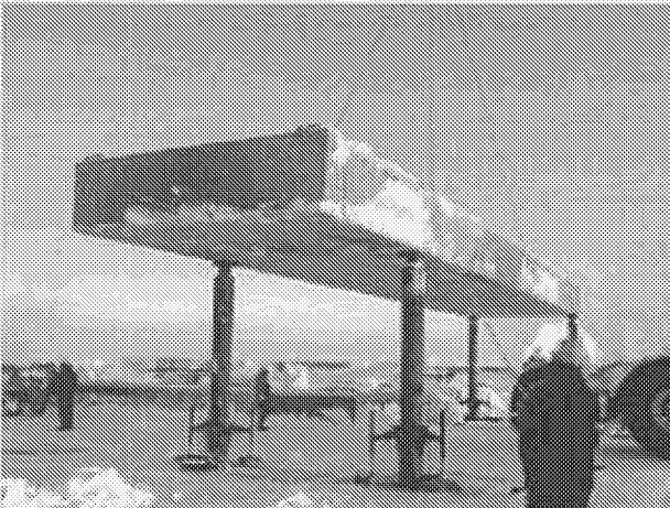
Figure A-3. Setting the First Platform Module
