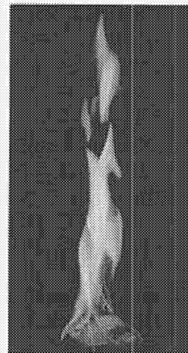
Figure 2. Methane Hydrate
