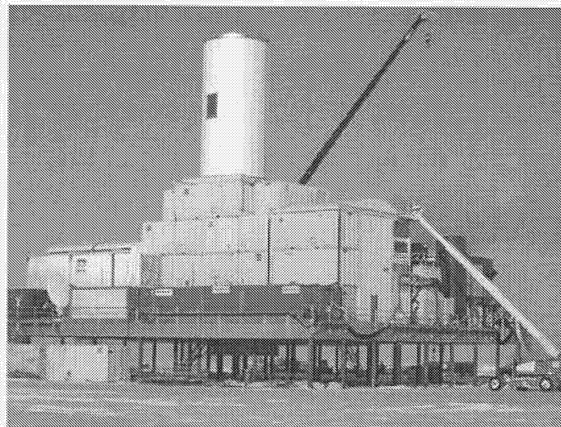
Figure 10. Arctic Platform at Hot Ice #1
