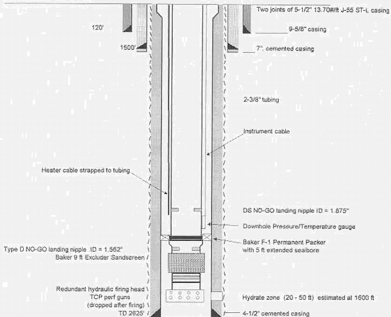
Figure B-1. Hot Ice #1 Completion
