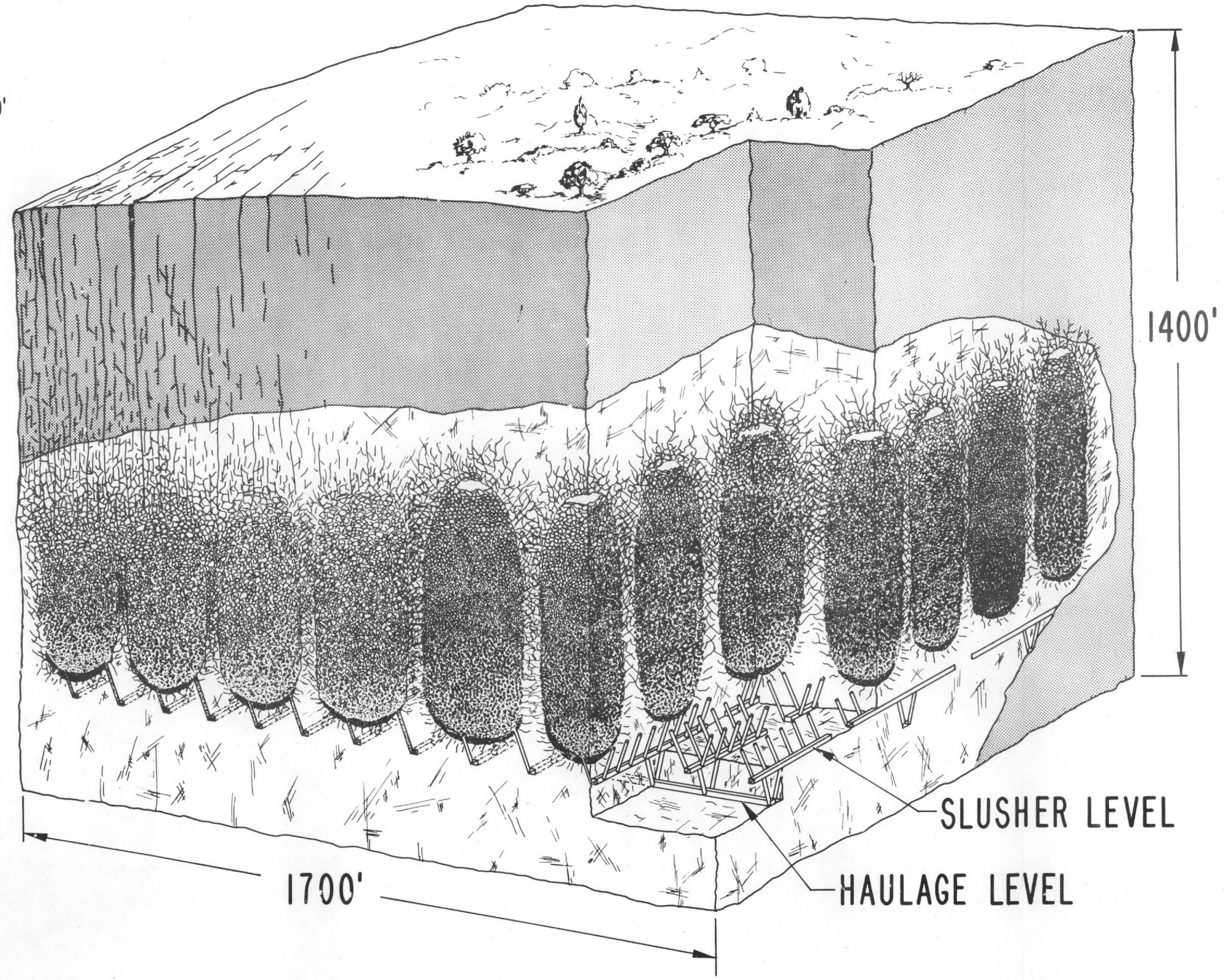
Fig. 8. Nuclear caving mine.
