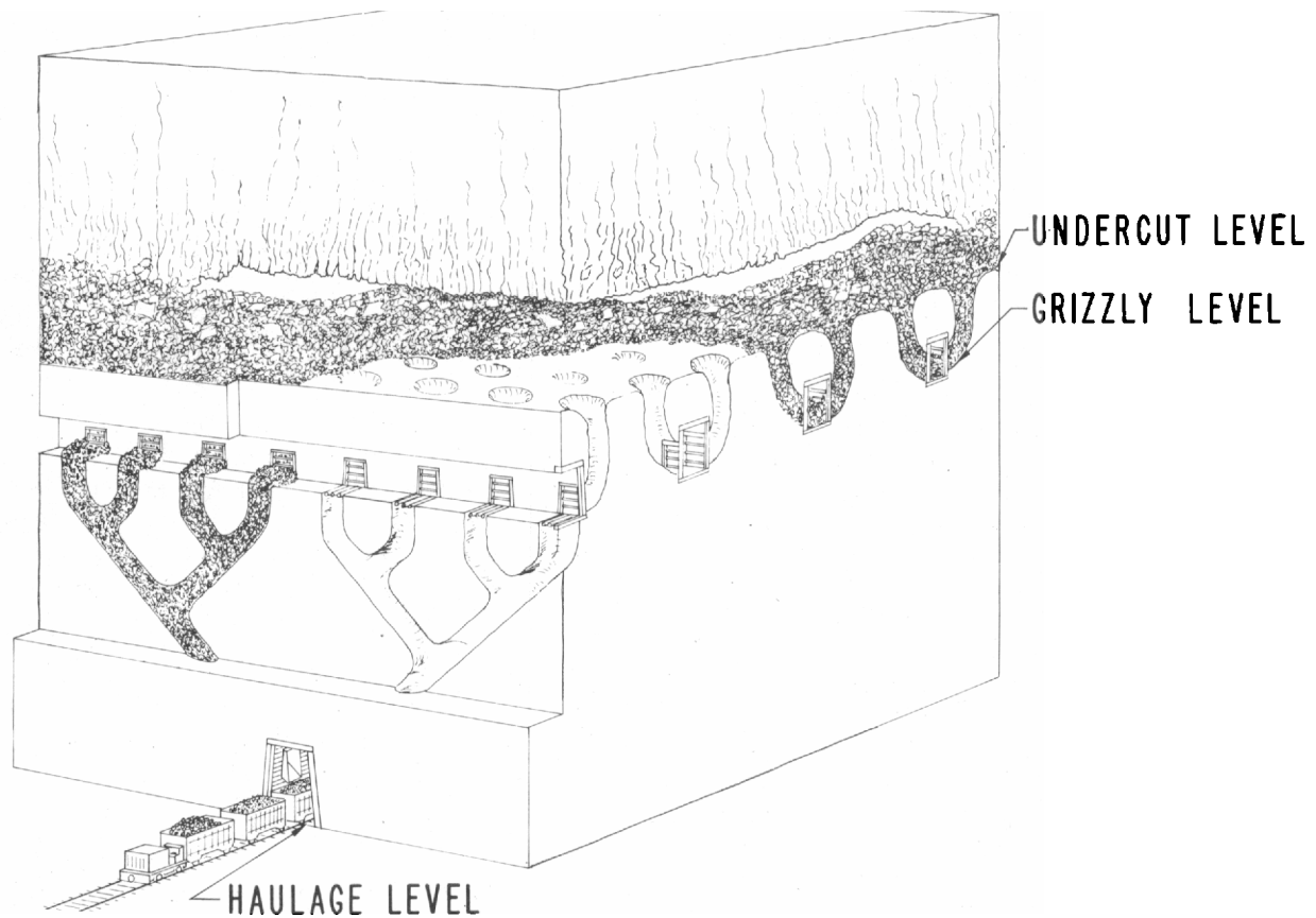
Fig. 6. Conventional grizzly control gravity transfer.
