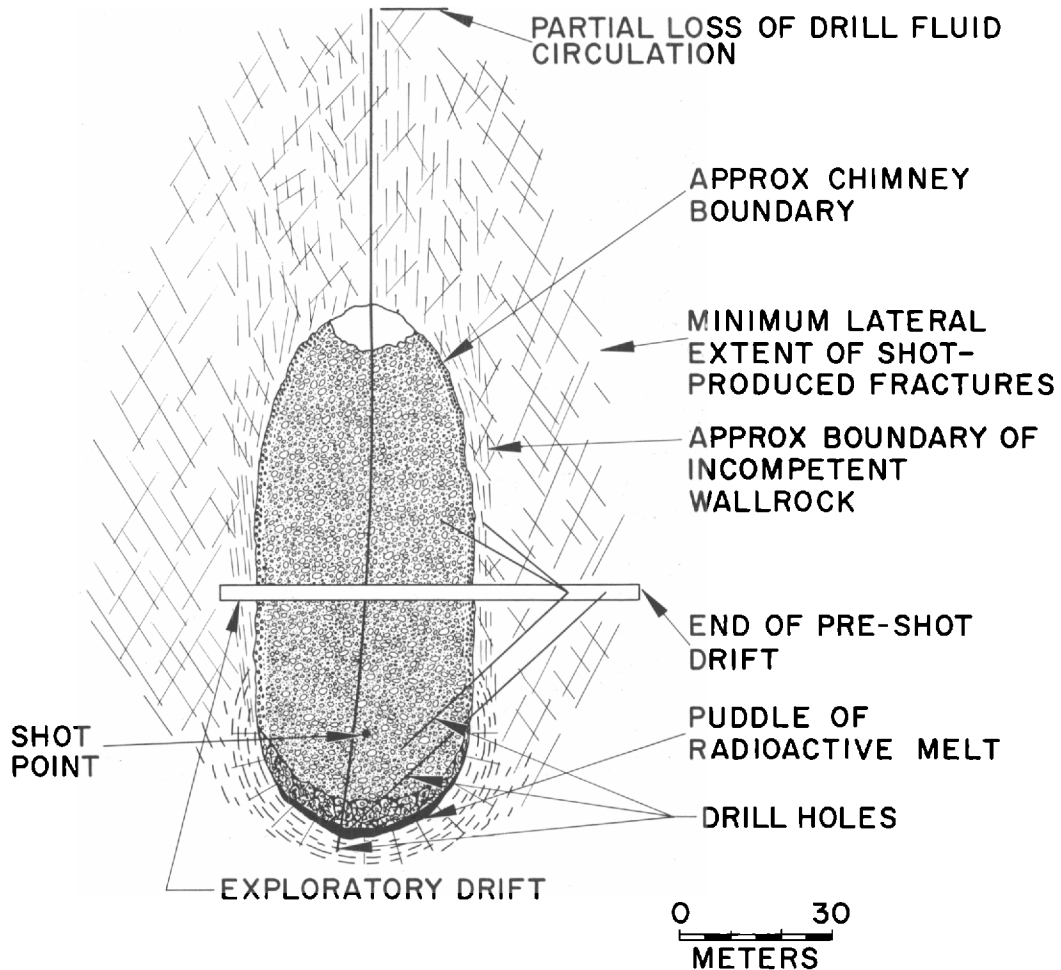
Fig. 1. Hardhat chimney.
