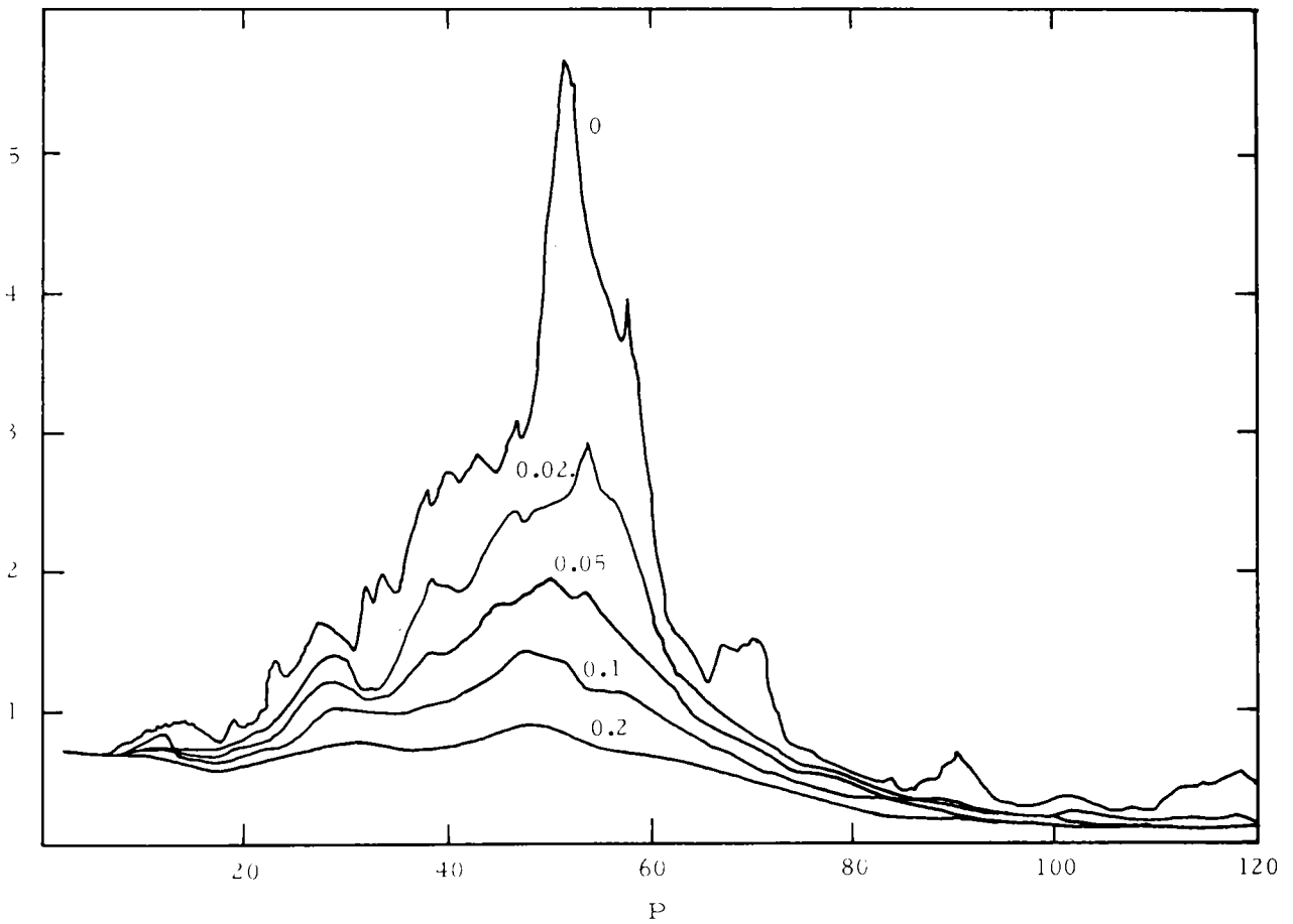
Fig. 6. Relative velocity spectrum for one GNOME accelerogram. Damping - 0, 2, 5, 10, 20% critical. S_v in units of 10 cm/sec. Frequency P in rad/sec.
