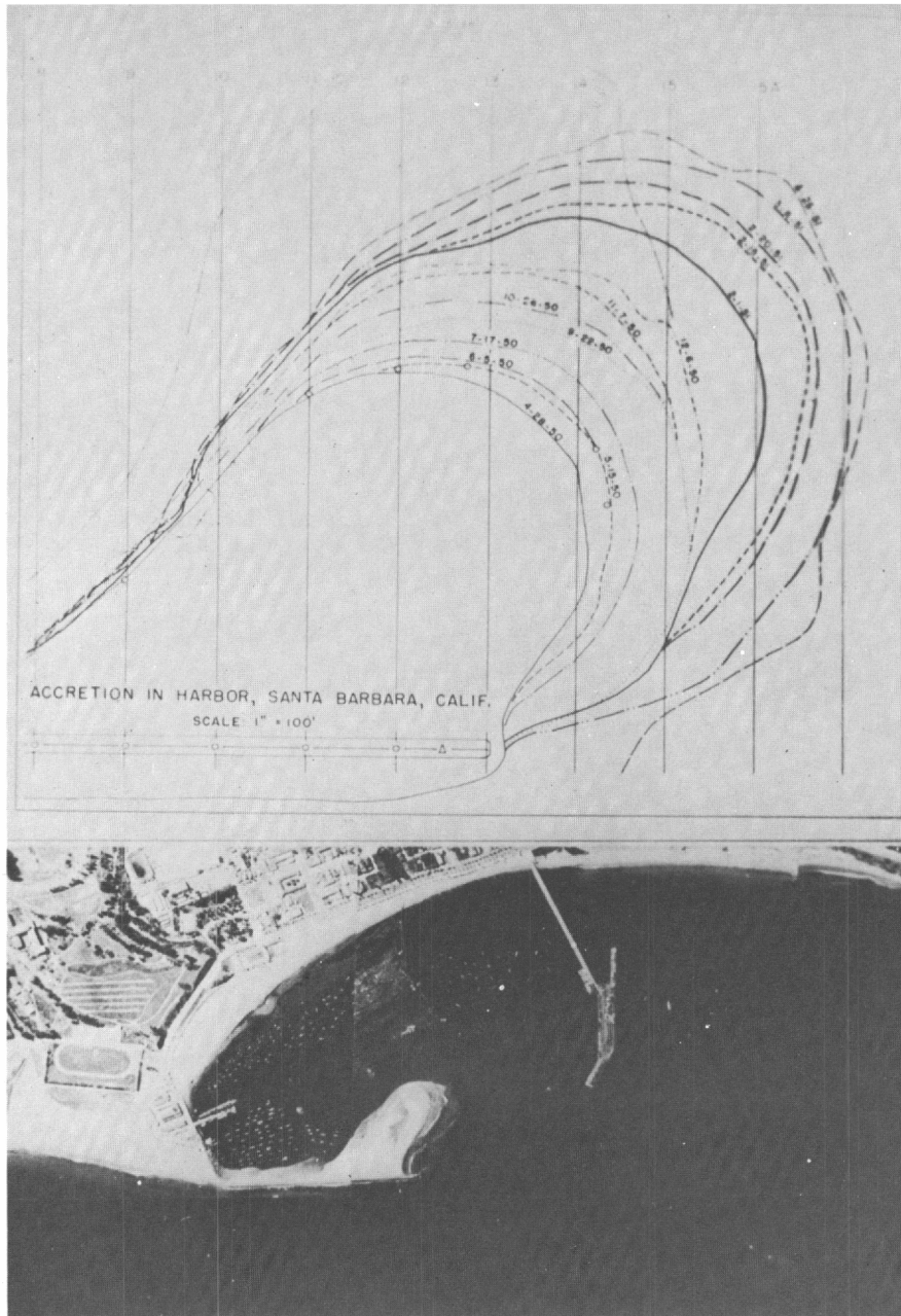
Fig. 4. Santa Barbara, California, has a serious sand and beach problem created by the construction of a breakwater. Sand which moves eastward along the coast (left to right) under the influence of the prevailing westerly waves is unable to pass the breakwater and deposits in its quiet lee. Besides blocking the harbor, this starves the beaches at the right of the picture, which retreat rapidly. The upper diagram shows successive stages in the growth of the sand spit. The sewage, lower right, shows that currents exist even on this calm day.
