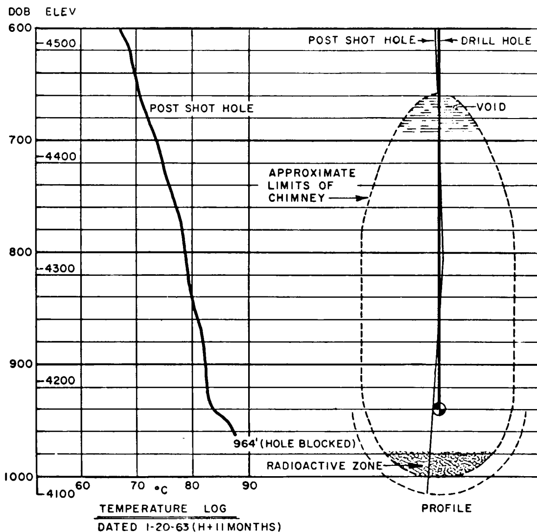
Fig. 7. Hardhat temperature profile.
