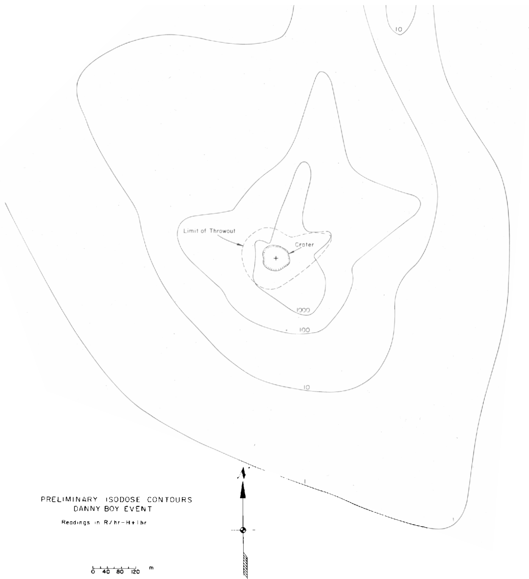
Fig. 3. Danny Boy close-in fallout pattern.
