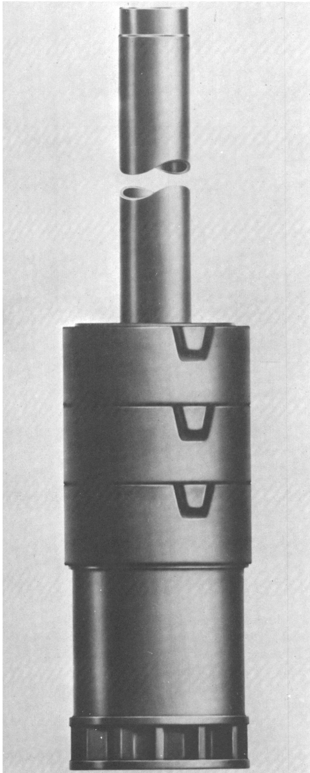
Fig. 14. View of a stacked "do-nut" drill collar assembly. Photo-Hughes Tool Co.
