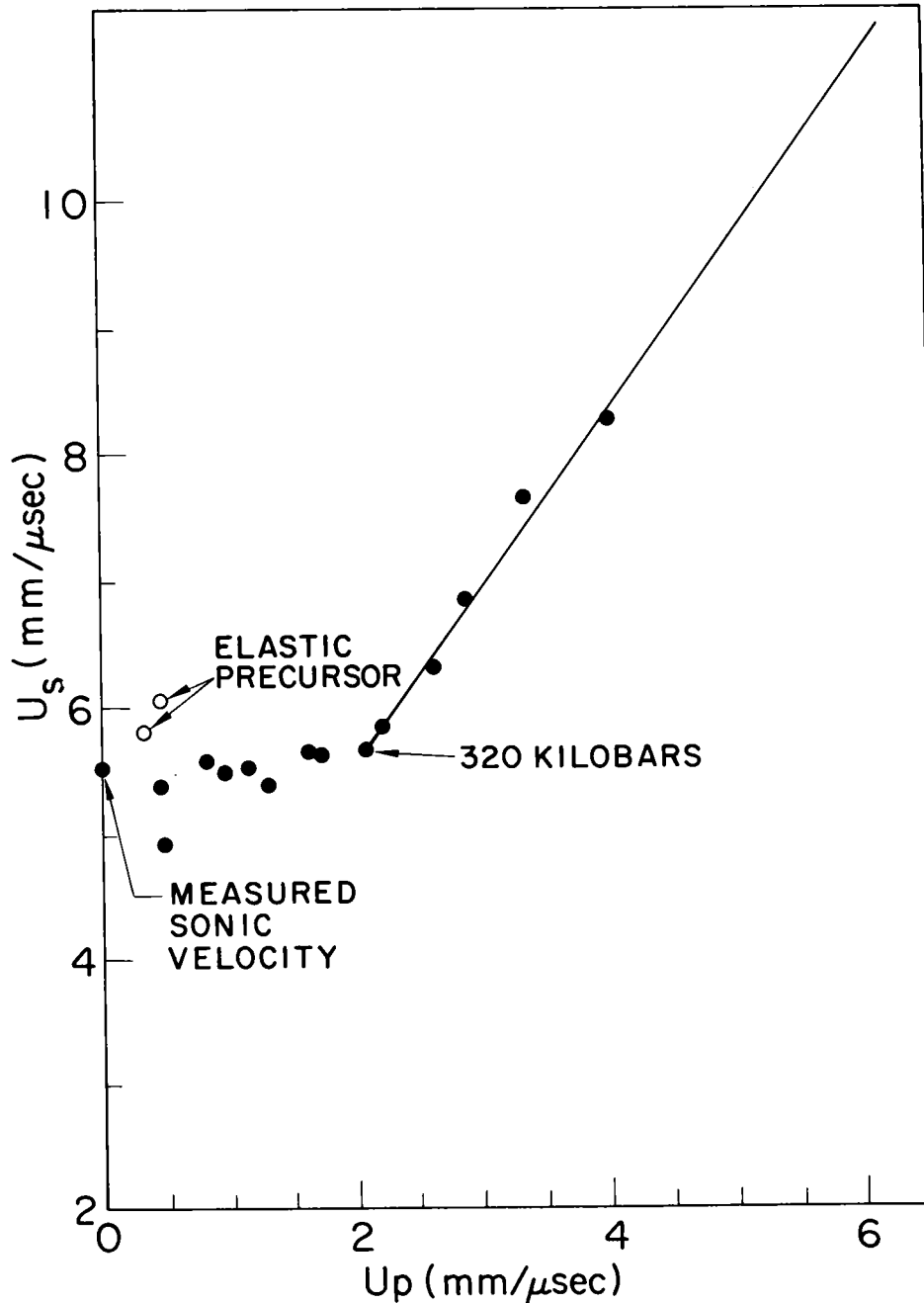
Fig. 3. Hugoniot measurements for granite.
