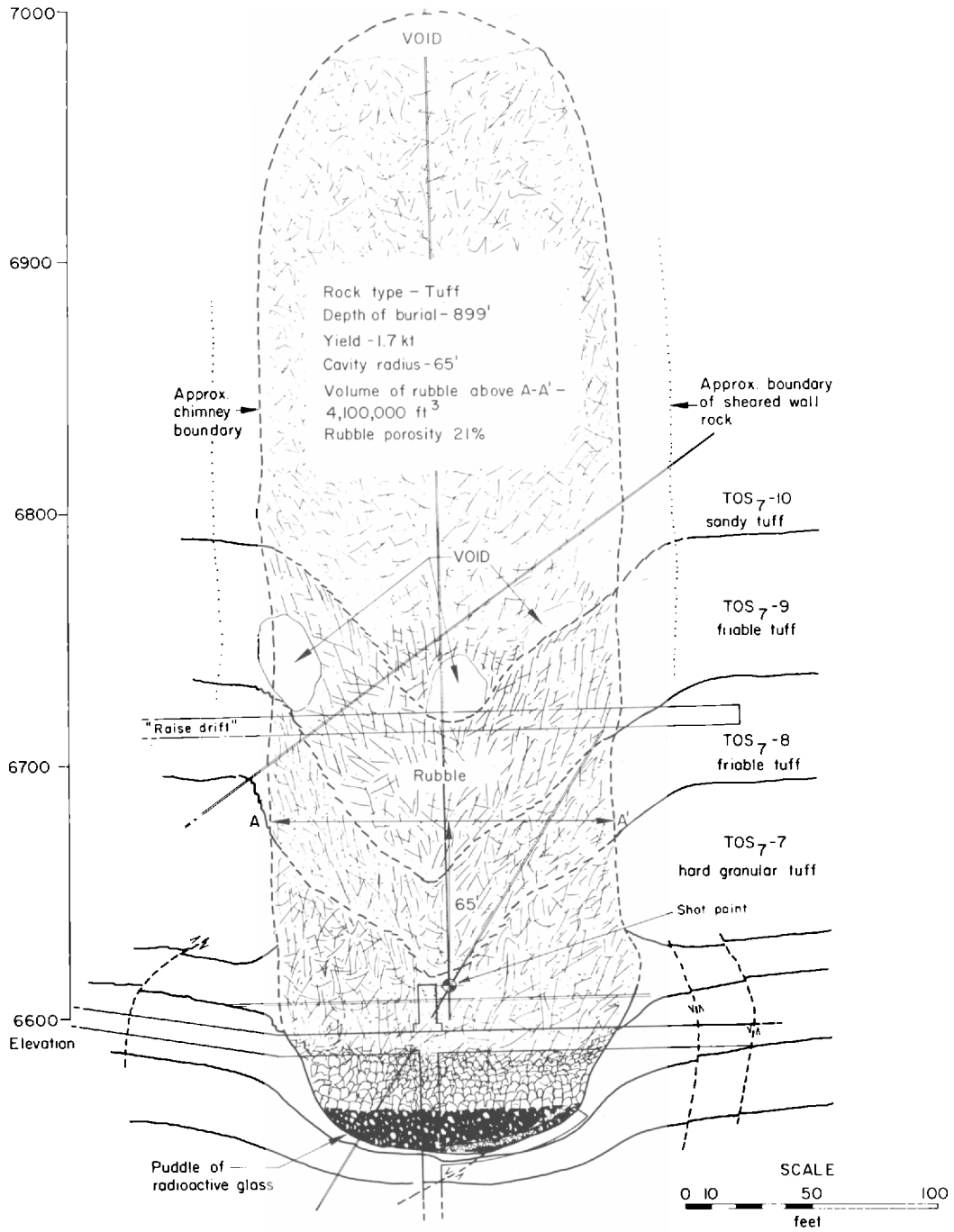
Fig. 12. Rainier schematic cross section.
