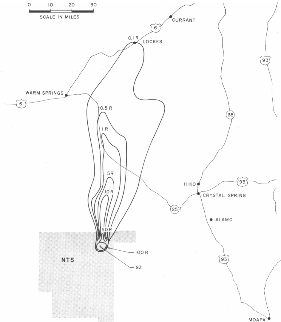
SEDAN FALLOUT PATTERN ISO-DOSE CONTOURS INFINITE DOSE FROM ARRIVAL
