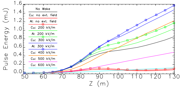
Figure 7: Pulse energy vs. z for 200-pC bunch charge propagating in Al & Cu vacuum chambers for various wake compensation undulator strength tapers.
