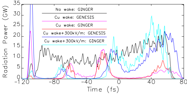
Figure 4: Predicted instantaneous power (artificially smoothed to 1-fs resolution) at z = 100 m for a 1-nC bunch charge propagating in a Cu vacuum chamber with and without wake effects.
