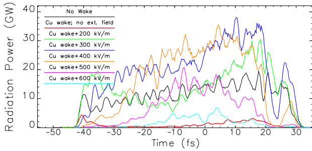
Figure 6: GINGER predictions for instantaneous power at z = 130 m for a 200-pC bunch charge propagating in a Cu vacuum chamber for various degrees of wake compensation tapers.
