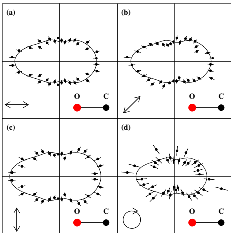
FIG. 3: Angular distribution of Auger electrons from the narrow 1\Sigma^+ line at 250.5 eV (B-state) (see Fig. 1). The orientation of the molecule is horizontal with the oxygen to the left as indicated. a-c linear polarized light, the polarization vector is indicated by the double arrow. (d) circular polarized light, propagating into the plane of the figure.
