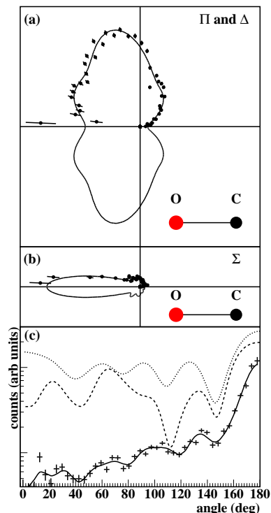
FIG. 4: Angular distribution of Auger electrons from \text{CO}^+ . (a) from region I Fig.1a, (b) region II Fig. 1a. (a) corresponds to the \text{CO}^+(1\Sigma^+) \rightarrow \text{CO}^{2+}(1\Delta, 3\Pi, 1\Pi) transition. b) corresponds to a \text{CO}^+(1\Sigma^+) \rightarrow \text{CO}^{2+}(1\Sigma) transition. c) same data as in b) 0 deg corresponds to emission in direction of the carbon. The full lines in all figures are a fit of Legendre polynomials to guide the eye. Other lines in c) are results of a multiple scattering calculation for an S electron wave starting at the carbon center in \text{CO}^{2+} . Dashed: both vacancies in the \text{CO}^{2+} at C(2p), dotted: one vacancy each at C(2p) and O(2p). The absolute height of the calculation is arbitrary.
