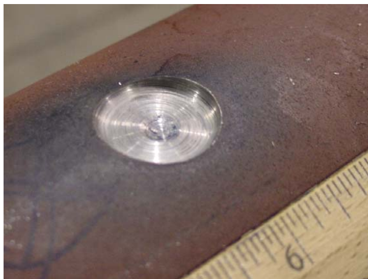
Figure 13 - Short, Deep Simulated Corrosion Damage
