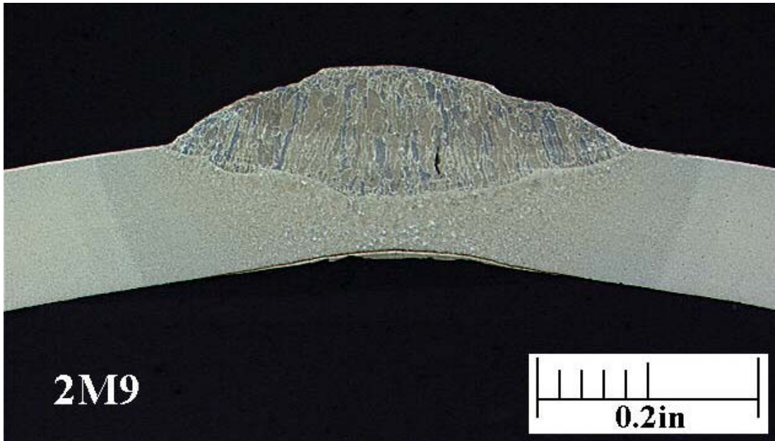
Figure 103 - Metallographic Section through Weld 2M9 (middle weld shown in Figure 101 and Figure 102)
