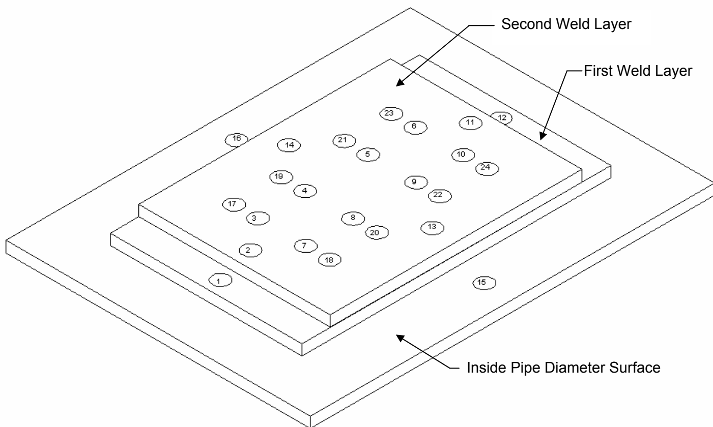
Figure 94 - Ultrasonic Thickness Measurement Locations on Weld Deposition Repair
