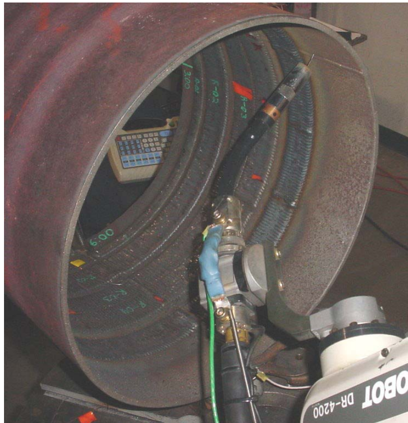
Figure 34 - OTC Robot Arm and Torch
