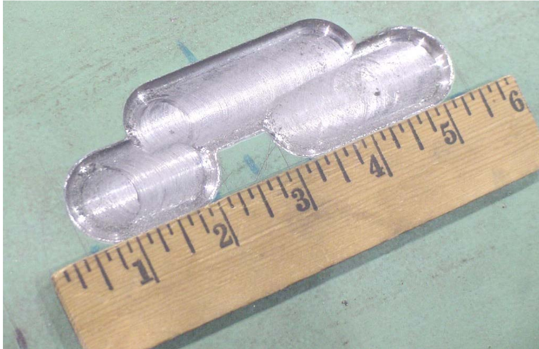
Figure 88 - Selected Configuration of Simulated Damage for 508 mm (20 in.) Diameter Pipe Sections
