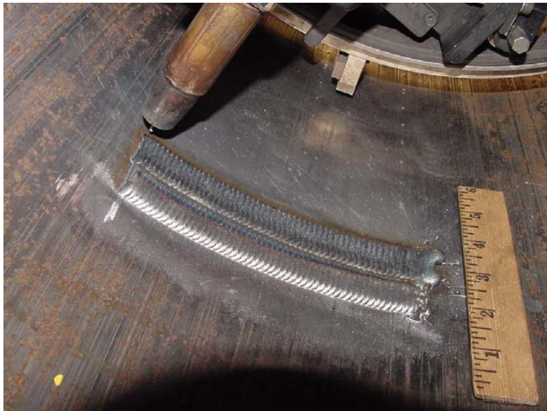
Figure 47 - Second Pass of First Layer of Deposited Weld Metal on Inside Pipe Diameter
