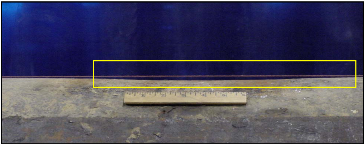
Figure 97 - Profile of Dent in Outside Pipe Surface After Internal Weld Deposition Repair
