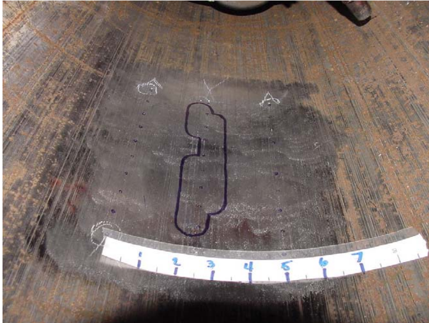
Figure 45 - Outline of Simulated Corrosion on Inside Diameter of Pipe Section
