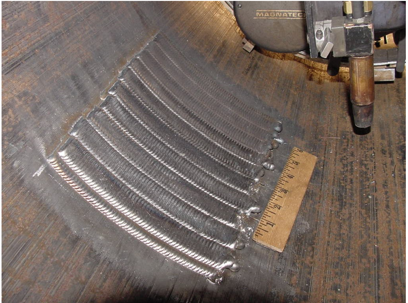
Figure 51 - Finished Second Layer of Deposited Weld Metal on Inside Pipe Diameter
