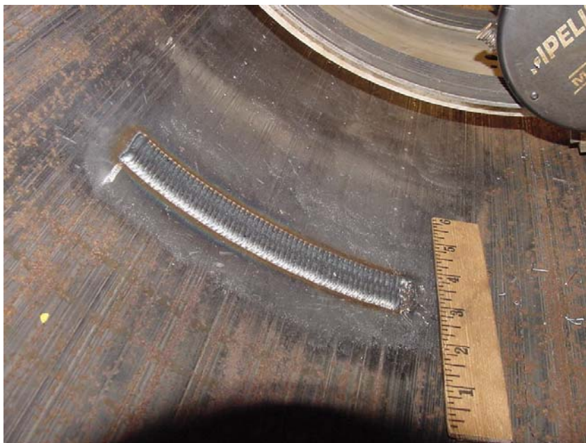
Figure 46 - First Pass of First Layer of Deposited Weld Metal on Inside Pipe Diameter
