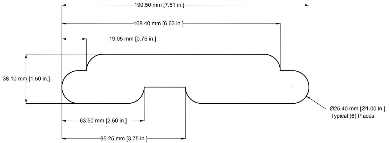
Figure 40 - Dimensions of Simulated Corrosion on 558.80 mm (22 in.) Pipe
