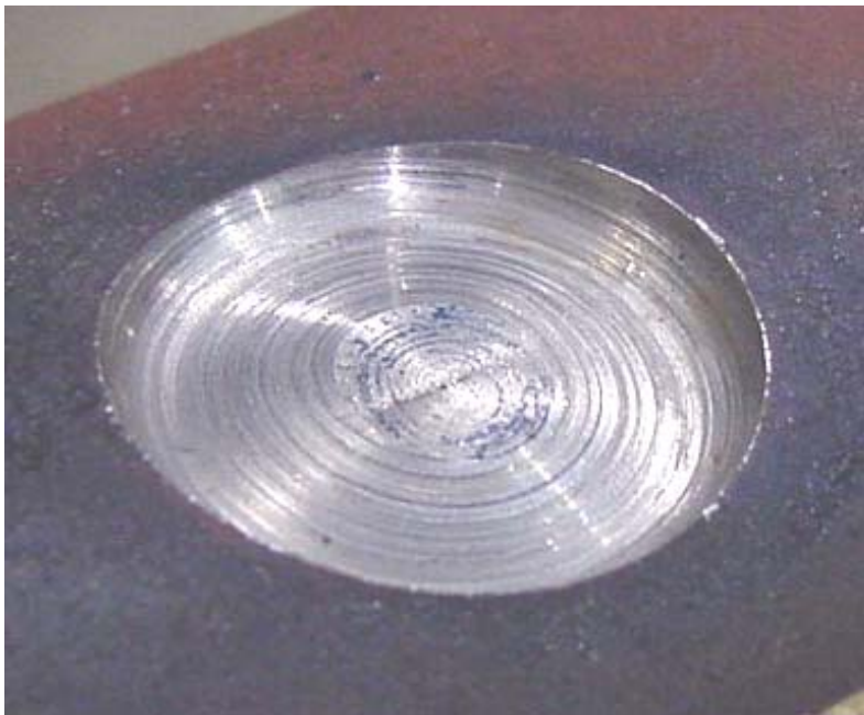
Figure 77 - Pipe Section with Short, Deep Simulated Corrosion Damage – With Liner – Following Hydrostatic Pressure Test
