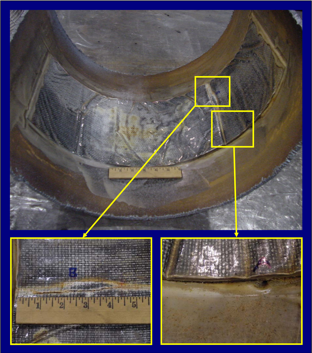
Figure 118 - Pressure Bandage Style Carbon Fiber Patch with Failure Locations
