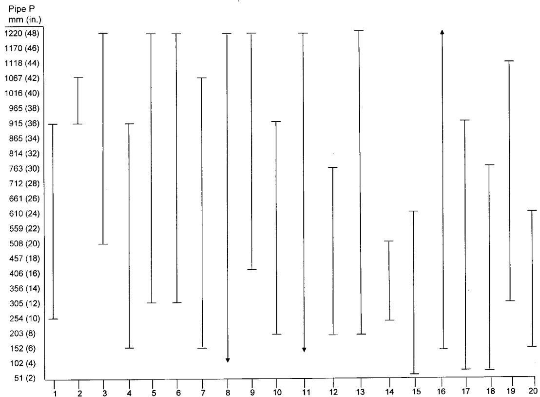
Figure 57 - Range of Pipe Diameters Used
