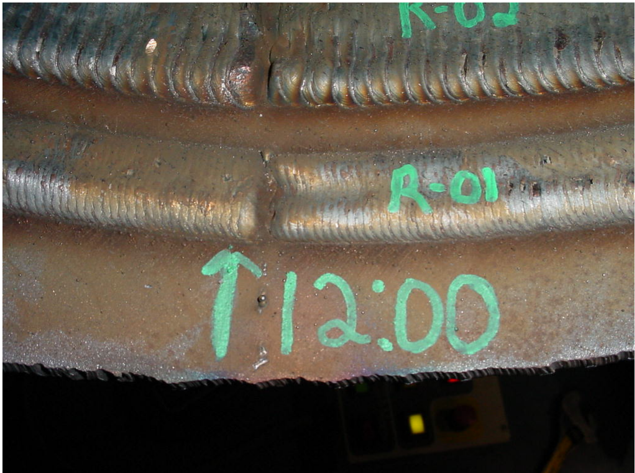
Figure 83 - Test R-01 at 12:00 Showing Poor Stop-Start Tie-In
