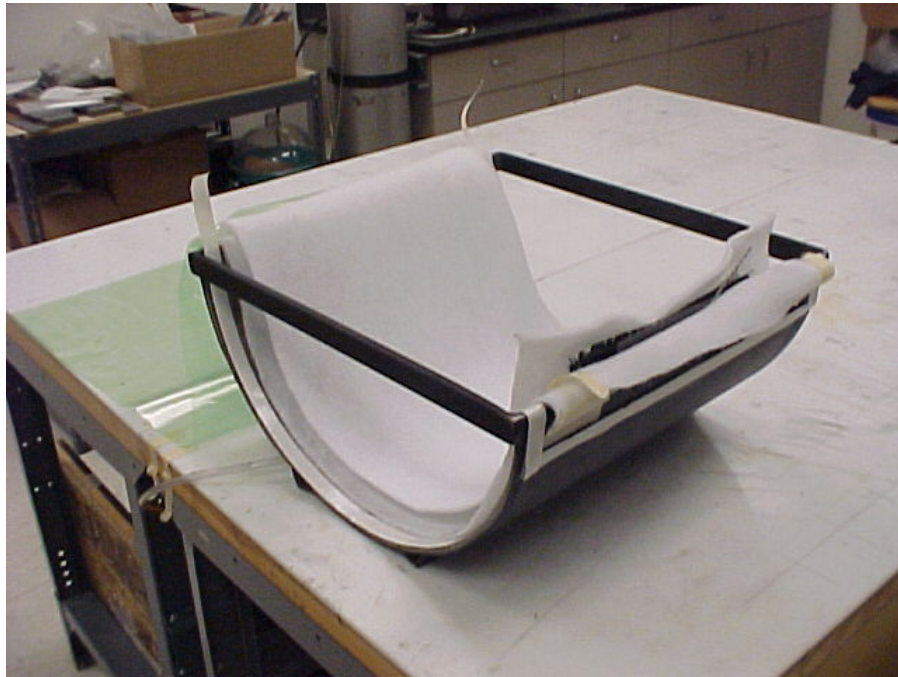
Figure 20 - Mylar Top Shown Draped (Top Breather Draped Next Over Pack)
