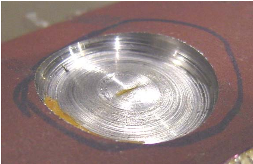
Figure 76 - Pipe Section with Short, Deep Simulated Corrosion Damage – Without Liner – Following Hydrostatic Pressure Test
