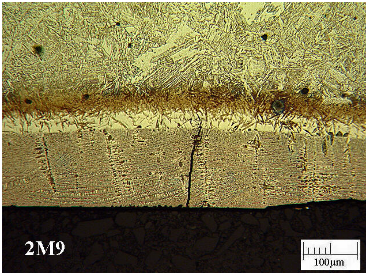
Figure 105 - Cracks in Eutectic Iron Layer of Metallographic Section Shown in Figure 104
