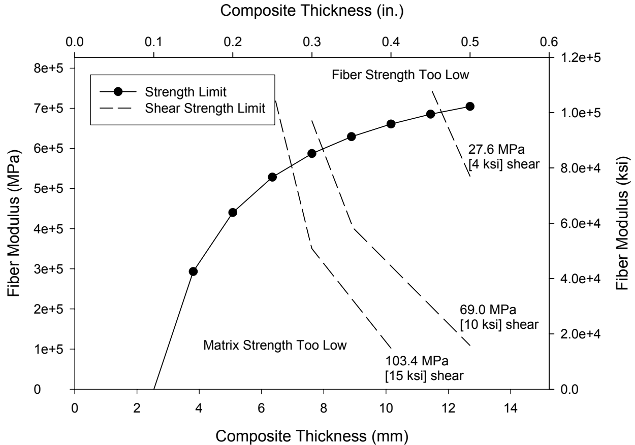
Figure 90 - Design Space for Composite Liner
