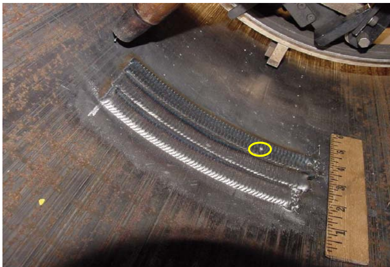
Figure 48 - Third Pass of First Layer of Deposited Weld Metal on Inside Pipe Diameter
