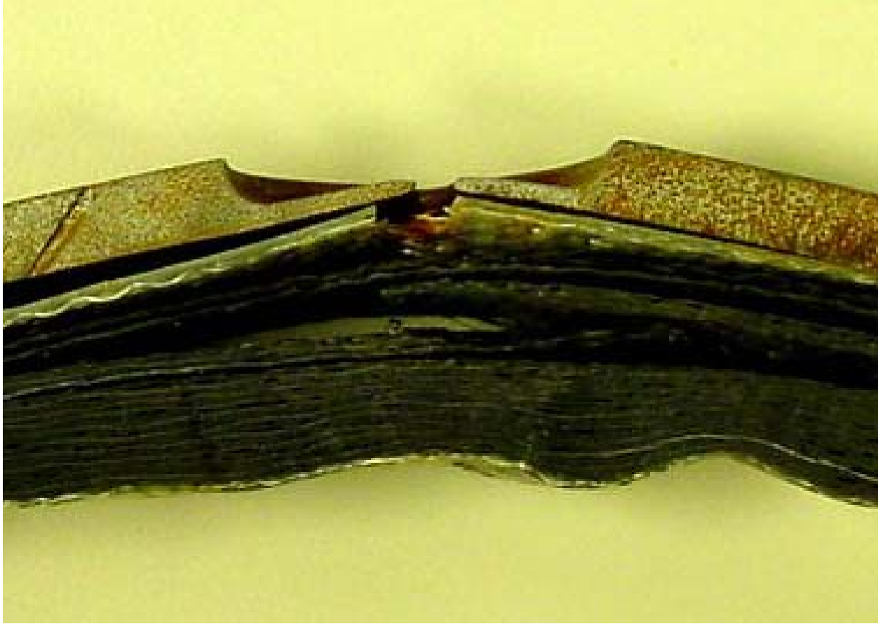
Figure 120 - Disbondment Between Pipe and Patch at Pipe Failure Site
