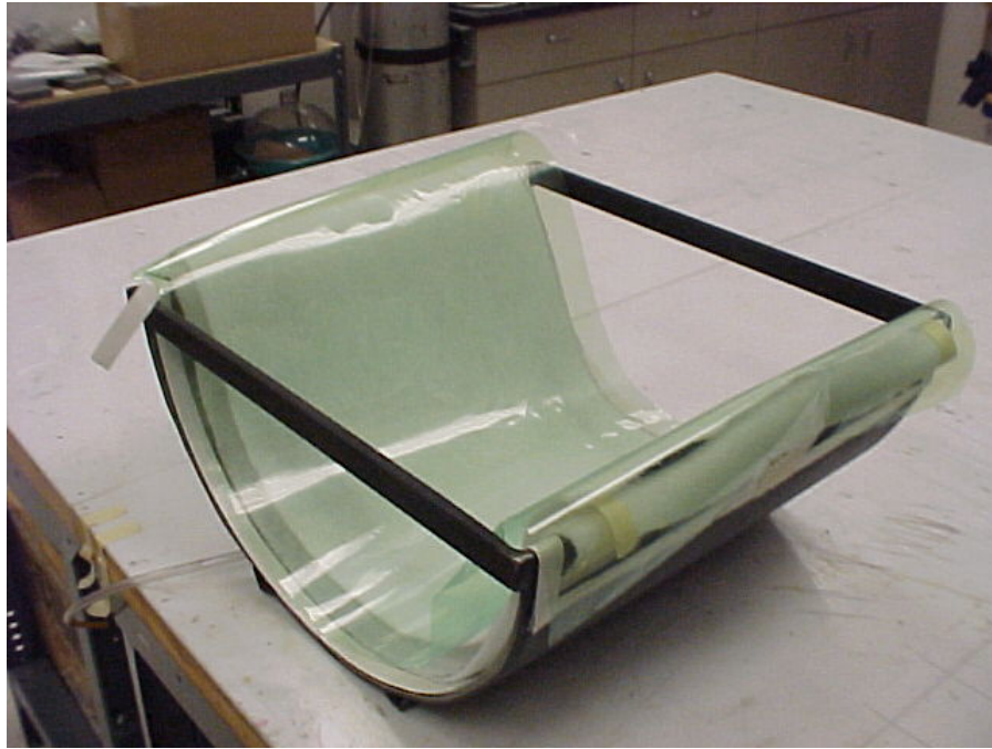
Figure 21 - Vacuum Bag Film Draped Over Entire Pack
