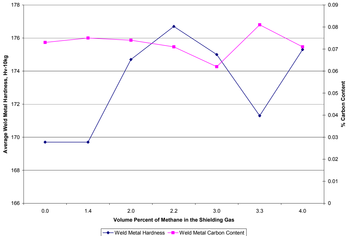
Figure 106 - Graphical Representation of Table 19 Hardness Values and Carbon Content
