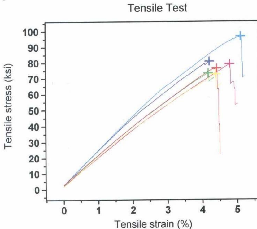
Figure 80 - Tensile Testing Results for Glass/Polypropylene Liner Material
