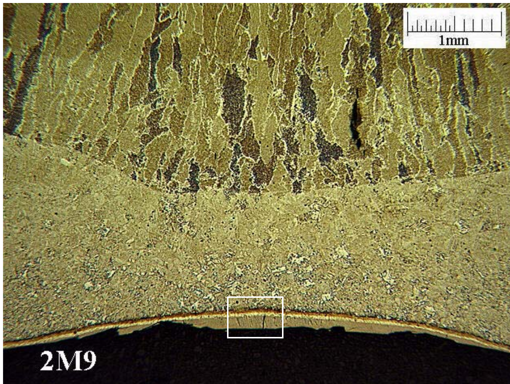
Figure 104 - Eutectic Iron Layer at Inside Surface of Section through Weld 2M9
