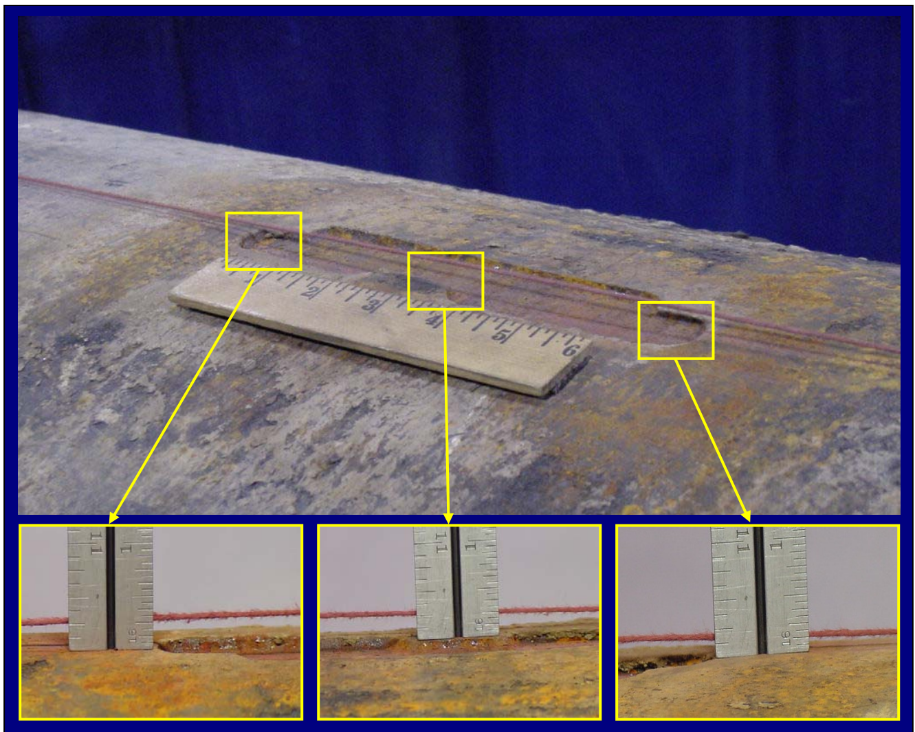
Figure 98 - Magnified Pictures of Dent at Ends and Middle of Simulated Damage
