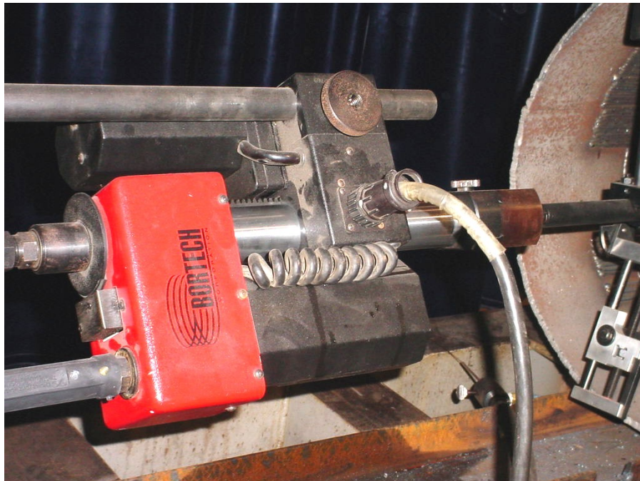
Figure 30 - Bortech Motion Mechanism for Continuous Spiral Deposition
