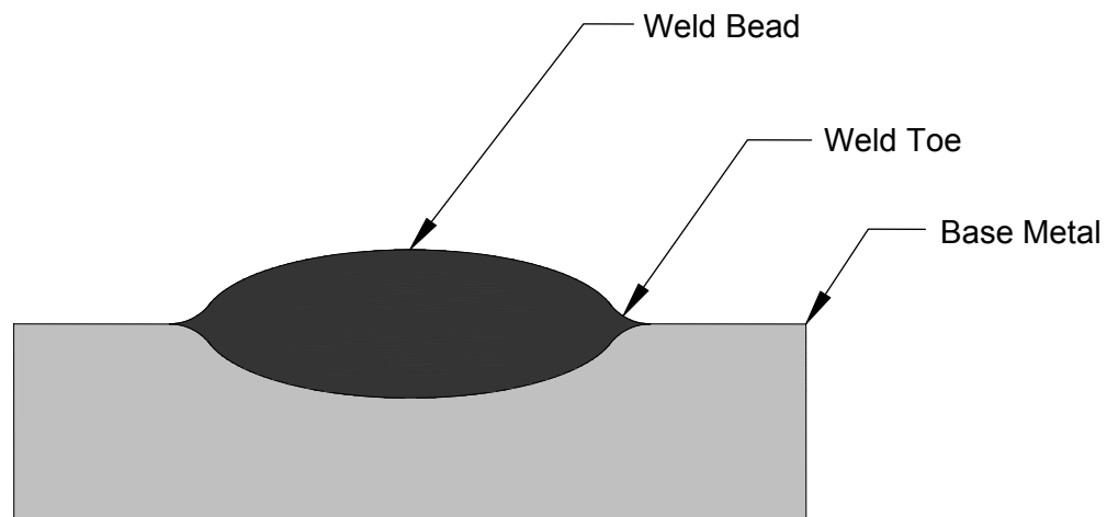
Figure 81 - Weld Bead Shape Diagram
