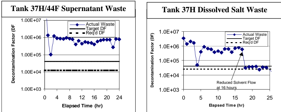
FIGURE 3. Waste Decontamination as a Function of Elapsed Time
