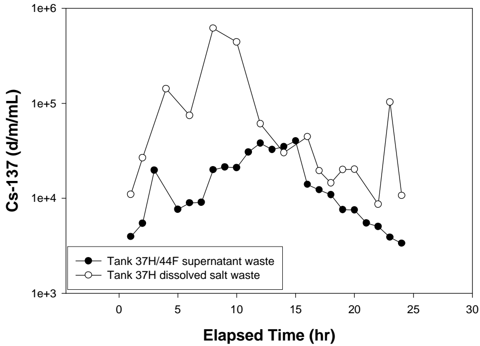
FIGURE 4. Cesium Concentration in the Solvent as a Function of Elapsed Time.
