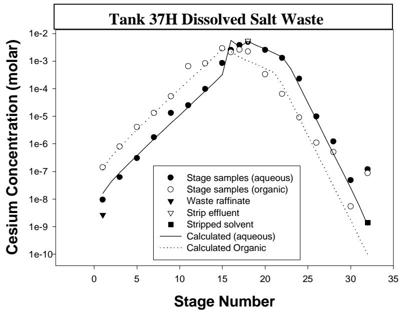
FIGURE 6. Comparison of Stage Sample Data and SASSE Calculated Concentrations
