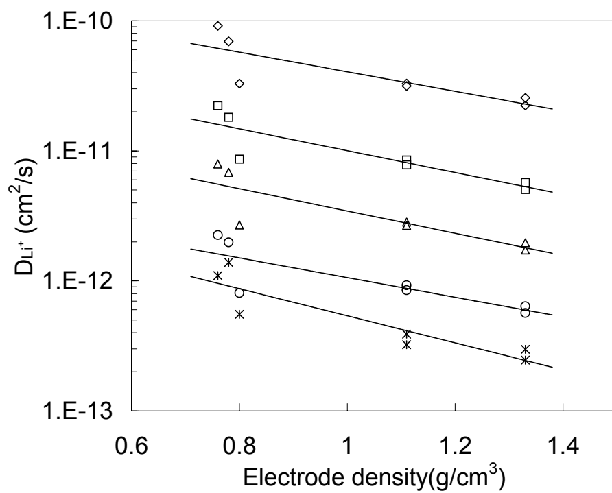
Fig. 11. Chemical diffusion coefficient of Li ion on x in Li_xC_6 calculated from EIS; ( \diamond ) x=0.1 , ( \square ) x=0.2 , ( \triangle ) x=0.3 , ( \circ ) x=0.4 , ( * ) x=0.6
