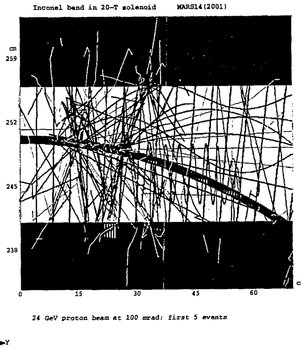
Figure 7. MARS simulation of secondary particle production from 5 interactions of 24 GeV protons in an inconel band target.
