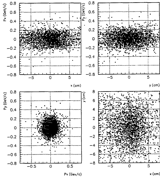
24 GeV protons on inconel band target ( \alpha_p=0.1 ) at the exit of a 20T solenoid
