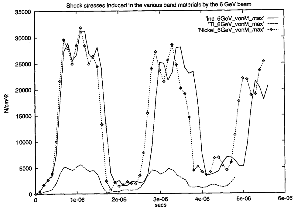
Figure 13. Same as figure 12. but for an incident bunch of 5 \times 10^{13} 24 GeV protons.
