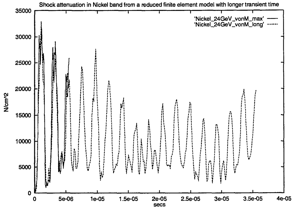
Figure 15. Similar to figure 13 for 5 \times 10^{13} 24 GeV protons on a nickel target, but extended to larger time values to show the dissipation of the shock stresses after multiple reflections from the band surfaces.
