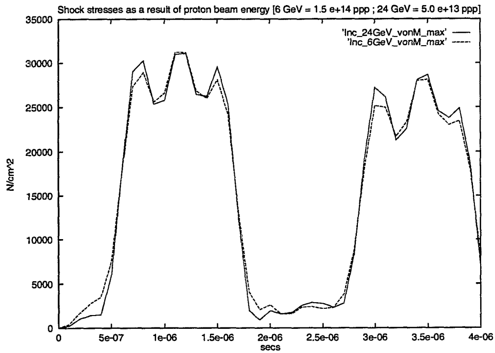
Figure 14. Similar to figures 12 and 13 for the inconel target, showing the close correspondence in the stress time development for 6 GeV and 24 GeV proton beams.
