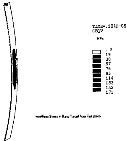
Figure 11. Predicted von Mises stress distribution for an inconel target band at one microsecond after exposure to an instantaneous proton bunch of 1.7 \times 10^{13} 24 GeV protons. This is a smaller bunch charge than would be typical for muon colliders; the distribution of stress values will scale in approximate proportion to the bunch charge in the linear regime before the material's fatigue strength is exceeded.
