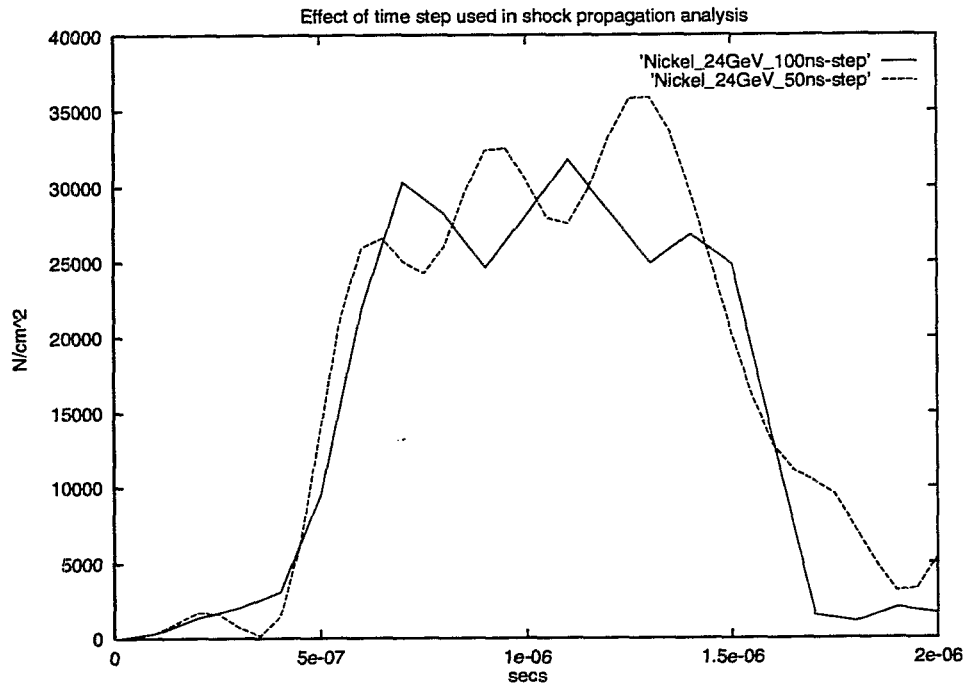
Figure 16. Similar to figure 13 for 5 \times 10^{13} 24 GeV protons on a nickel target but for both 50 ns and 100 ns time steps in the ANSYS simulation. The reasonable agreement between the two curves suggests that the normal 100 ns step size is adequately short for approximate stress predictions.
