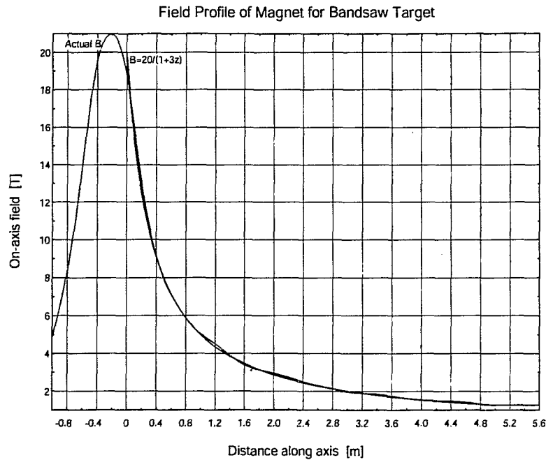
Figure 4. The on-axis magnetic field profile in the solenoidal capture channel. The plot shows, nearly superimposed, both the actual field and the “ideal” field profile it was fitted to.
