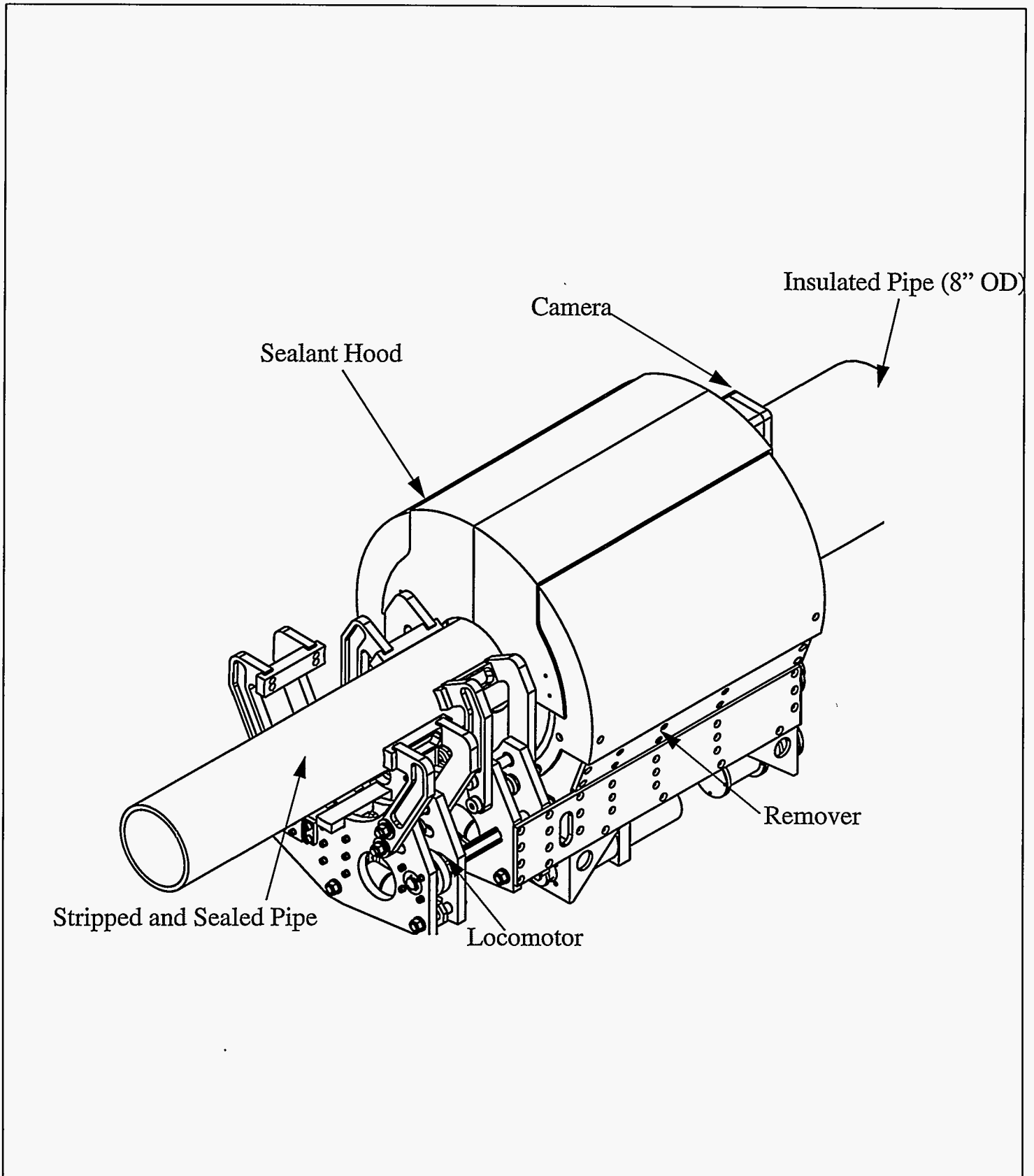
Figure 6-2: View of the BOA crawler robot developed in Phase I
