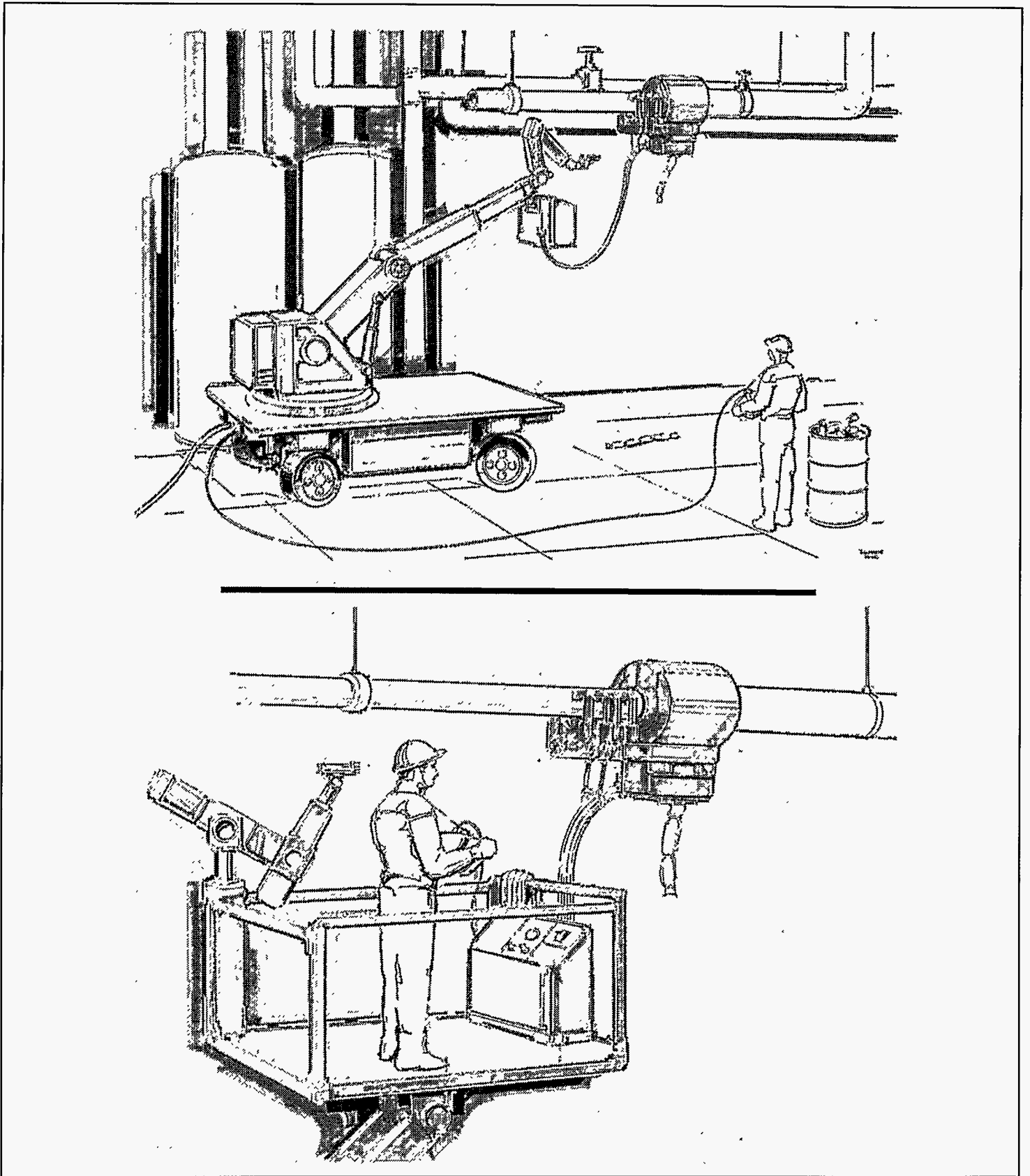
Figure 6-1 : Operational scenario for the pipe-asbestos insulation removal robot system in a fully robotic and human assistance modes, showing the asbestos removal and packaging actions in progress
