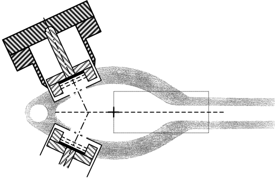
Figure 2: Mounting of two RFAs on a standard aluminum (Al) APS chamber, cross-sectional view. The RFA consists of two grids and a graphite-coated collector biased at +45V. The first grid is grounded and the second can be biased for electron energy selection [3,4].
