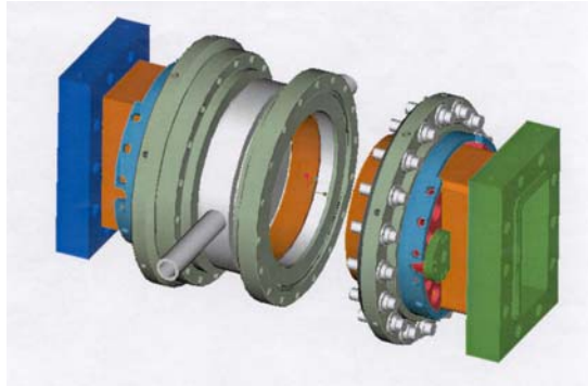
Figure 6: Disassembled 340 window.
