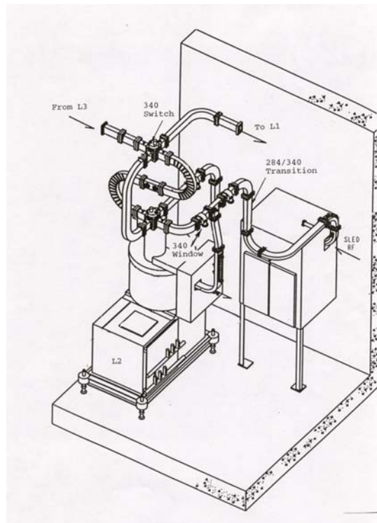
Figure 1: Waveguide switching system.
