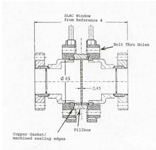
Figure 3: Pillbox style window.
