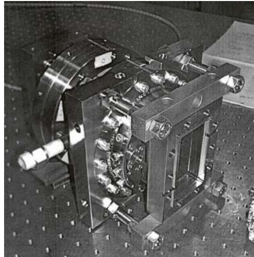
Figure 7: Weld fixture.
