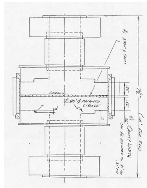
Figure 4: Initial investigative hardware.
