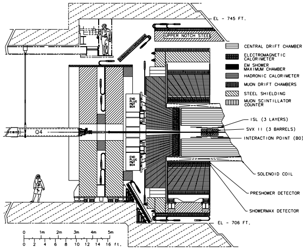
Fig. 1. The CDF Run 2 detector.
