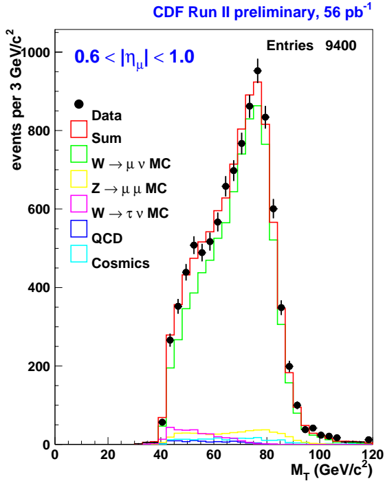
Fig. 2. W \rightarrow \mu\nu with the muon detected in CMX.
