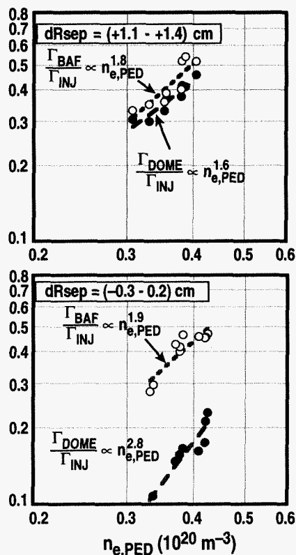
Fig. 4. \Gamma_{\text{BAF}}/\Gamma_{\text{INJ}} (open circles) and \Gamma_{\text{DOME}}/\Gamma_{\text{INJ}} (closed circles) depend strongly on the pedestal density for both (a) UDN: dR_{\text{sep}} = (1.1-1.4) cm and (b) BDN: dR_{\text{sep}} = (-0.3 - +0.2) cm.
