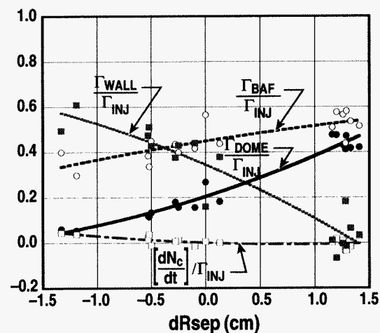
Fig. 3. \Gamma_{DOME} changed much more than \Gamma_{BAF} between dRsep = +1 to dRsep = -1 \text{ cm} . The values of \Gamma_{INJ} , \Gamma_{DOME} , \Gamma_{BAF} , and dN_C/dt were determined by measurement, while \Gamma_{WALL} was deduced from a particle balance. Each term is normalized to \Gamma_{INJ} . Parameter window: n_{e,PED} = (0.37\text{-}0.40) \times 10^{20} \text{ m}^{-3} and \Gamma_{INJ} = (9\text{-}13) \text{ torr l/s} .
