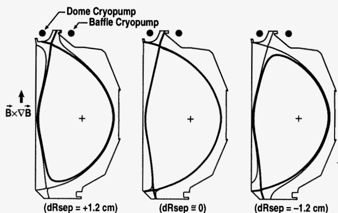
Fig. 1. The three basic equilibria used in this study: (a) DN biased toward the upper divertor ( dR_{sep} = +1.2 cm), (b) balanced DN ( dR_{sep} = 0 ), and (c) DN biased toward the lower divertor ( dR_{sep} = -1.2 cm). The “primary” (heavy) and “secondary” (light) divertor separatrices are shown. Characteristic parameters: I_P = 1.2 MA, B_T = 1.9 T, and P_{INJ} = 6-11 MW.
