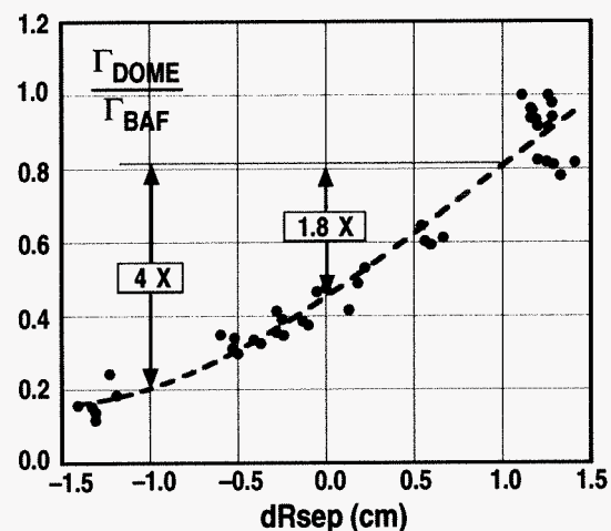
Fig. 2. The ratio \Gamma_{DOME}/\Gamma_{BAF} depends on dRsep .
