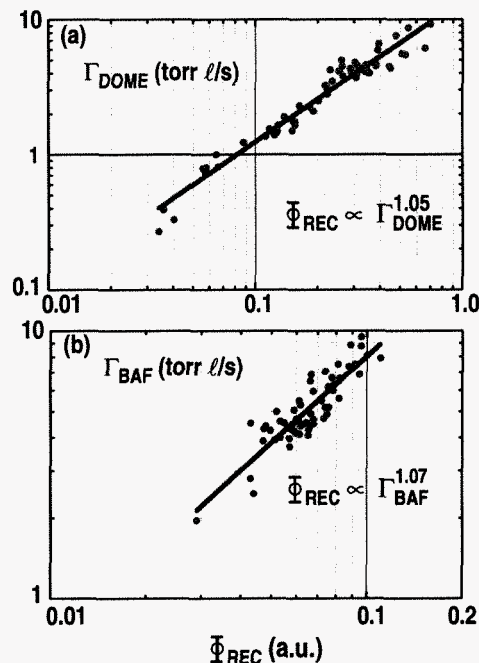
Fig. 5. (a) \Gamma_{\text{DOME}} and (b) \Gamma_{\text{BAF}} are plotted as a function of the recycling radiation [ \Phi_{\text{REC}} ] adjacent to the opening of the dome and baffle pumps, respectively.
