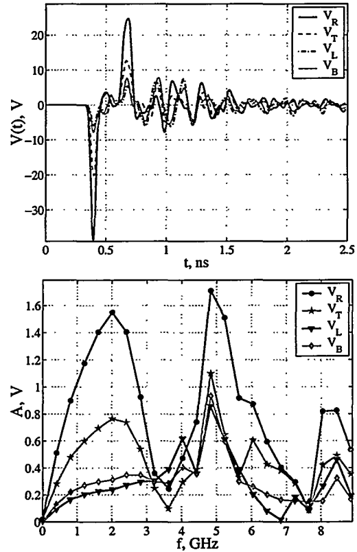
Figure 2: Signals on four BPM electrodes from a passing transversely displaced ( x=r_f/2 , y=r_f/4 ) bunch: (a) voltages versus time for one period 1/f_0=2.485 ns; (b) normalized Fourier amplitudes (V) vs frequency.
