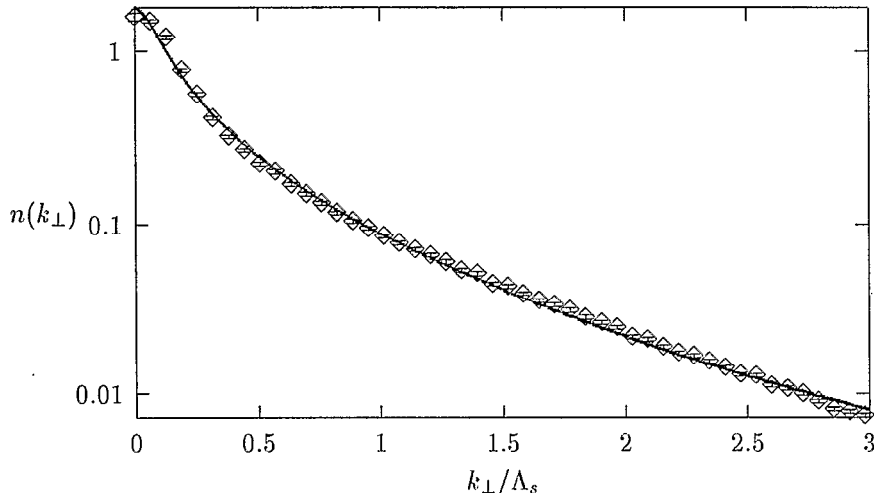
Figure 2: n(k_{\perp}) \equiv dN/L^2/d^2k_{\perp} as a function of the gluon momentum k_{\perp} for \Lambda_s L = 297 (diamonds). The solid line is a fit to Bose-Einstein distribution, corresponding to a gas of free particles at the inverse temperature \beta = (1.28 \pm 0.01)\Lambda_s and with the mass m = (0.092 \pm 0.003)\Lambda_s .
