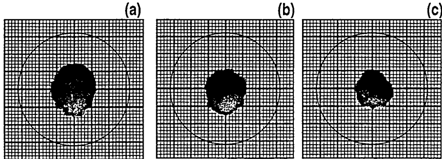
Fig. 3. The same rf beams shown in Fig 2 are shown in Fig. 3(a), (b), and (c) following reflection from pairs of mirrors especially designed to place a Gaussian waist with w/a = 0.64 at the input to the corrugated waveguides. The mirrors both focus and phase correct the beams produced by the gyrotrons. Thermally sensitive plotter paper is used to indicate the power profiles. The waveguide diameter, indicated by the circles, is 31.75 mm.
