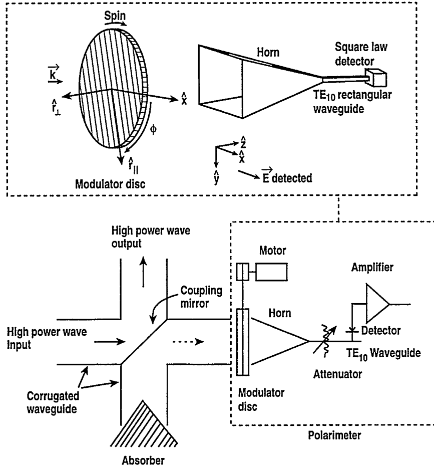
Fig. 6. Schematic diagram of the high power vacuum polarimeter. The rotating birefringent plate modulates the rf detected by a fundamental waveguide system which is then Fourier analyzed to obtain the polarization parameters.
