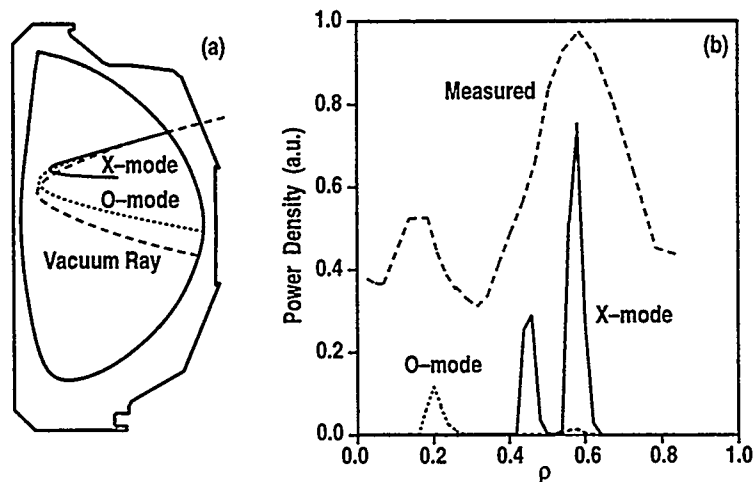
Fig. 4. The injected X-mode, O-mode, and the vacuum rf beam trajectories are shown projected to the poloidal plane of injection for a toroidal injection 19° off-perpendicular for current drive. The plasma second harmonic electron resonance is approximately on a vertical line at the major radius. The measured absorption profile has a peak associated with O-mode, although pure X-mode was intended to have been launched.
